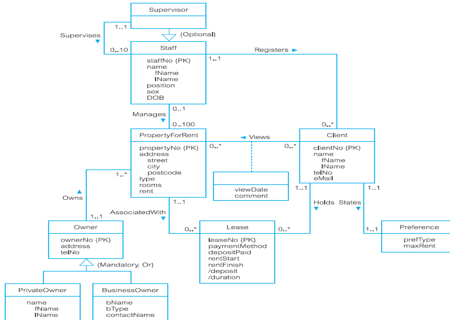
Figure 17.1 Conceptual data model for the StaffClient user views showing all attributes.
