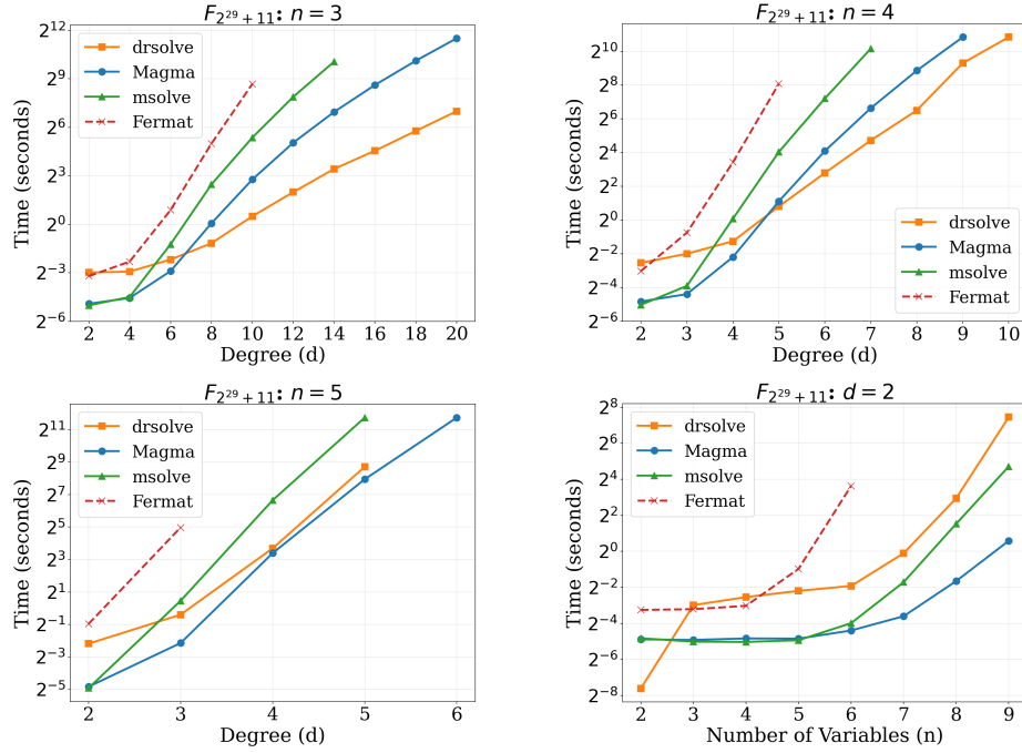
Fig. 2: Performance comparison (time in seconds) of DRSolve, Magma, msolve, and Fermat on randomly generated dense polynomial systems over \mathbb{F}_p with p = 2^{29} + 11 . The four panels show degree sweeps for n = 3, 4, 5 and a variable-count sweep for d = 2 ; here n denotes the number of variables (equal to the number of equations). A curve stops where the corresponding solver exceeded the time or memory budget of the benchmark.
