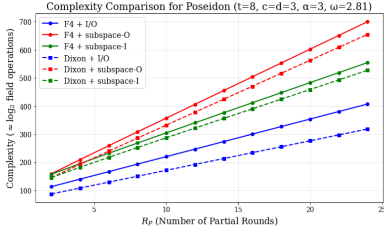
Fig. 3: Complexity comparison for POSEIDON and POSEIDON2, with the model parameters t = 8 , c = d = 3 , \alpha = 3 of [41]. Here \omega = 2.81 for all curves.
