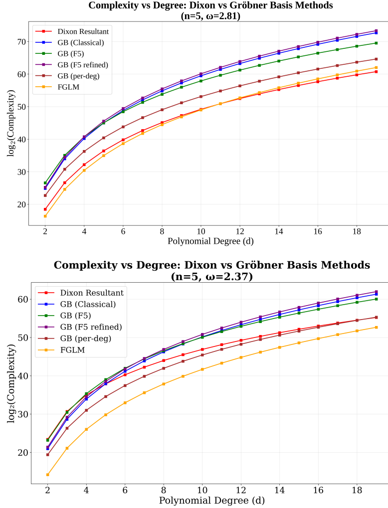
Figure 6 (continued). The bottom panel uses \omega = 2.37 . Since the asymptotic dominance of the final determinant sets in only for larger (n, d) than those plotted, the Dixon curve of this panel reports the maximum over the two symbolic stages, \max\{T_1^{\text{best}}, T_4^{\text{best}}\} , which over this range is governed by Step 1.
