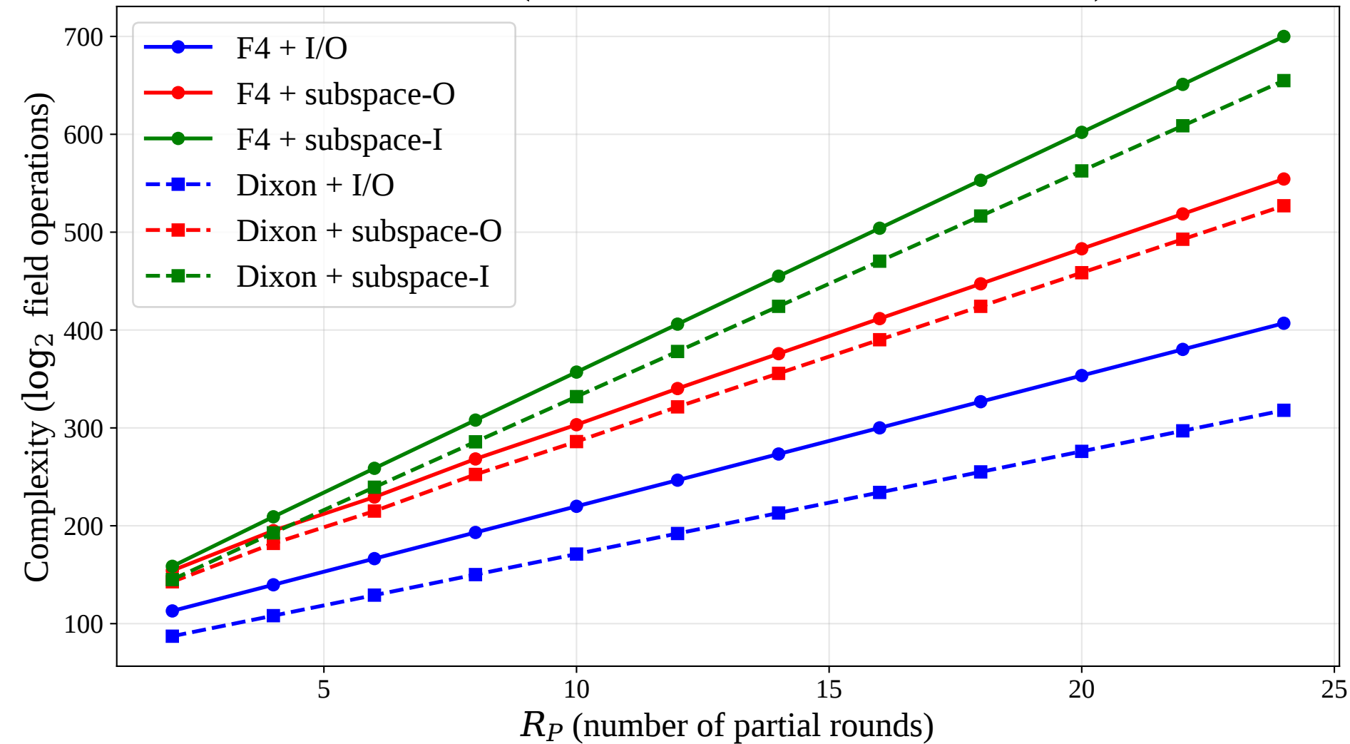
Poseidon2 ( t = 8, c = d = 3, \alpha = 3, \omega = 2.81 )
