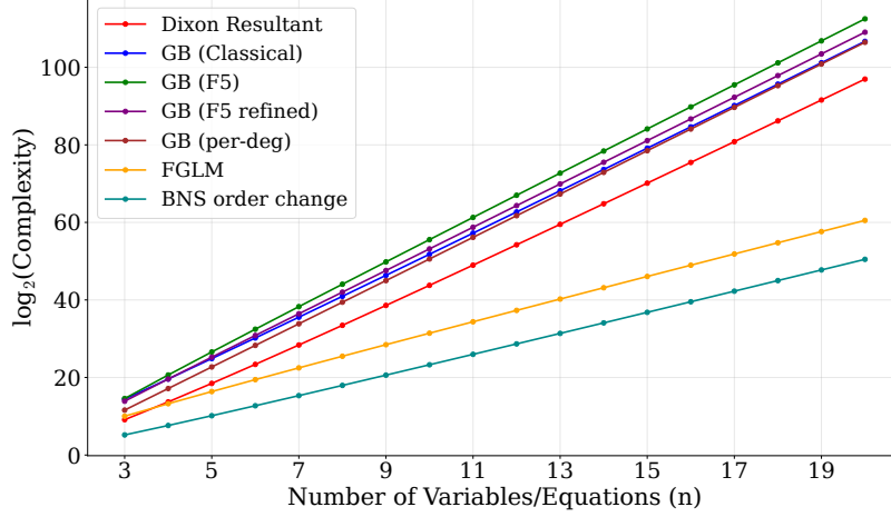
Complexity Comparison: Dixon vs Gröbner Basis Methods ( d=2, \omega=2.81 )
