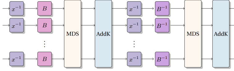
Fig. 10: Round function of Vision . (Figure from [22])
