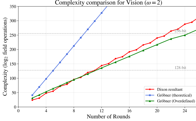
Fig. 4: Complexity comparison for Vision ( \omega = 2 for consistency with [60]).
