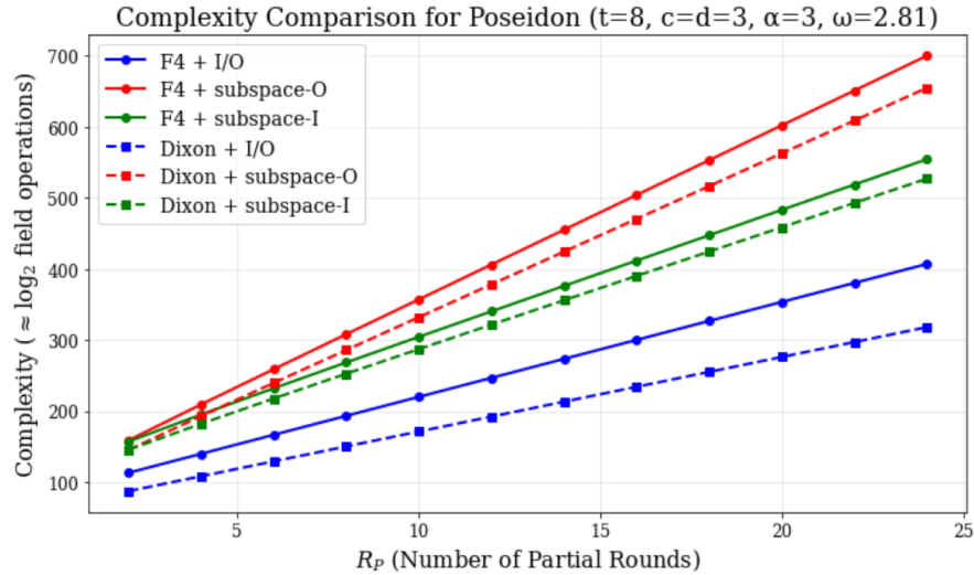
Fig. 3: Complexity comparison for POSEIDON and POSEIDON2, with the model parameters t = 8 , c = d = 3 , \alpha = 3 of [41]. Here \omega = 2.81 for all curves.
