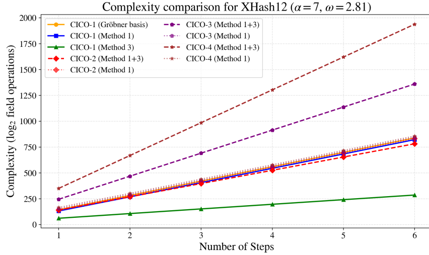
Fig. 5: Complexity comparison for XHash12, \omega = 2.81 .
