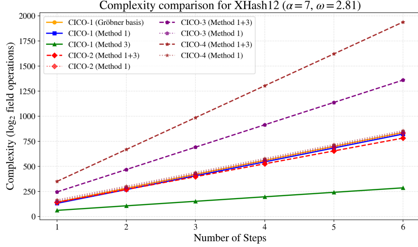
Fig. 5: Complexity comparison for \mathbf{XHash12} , \omega = 2.81 .
