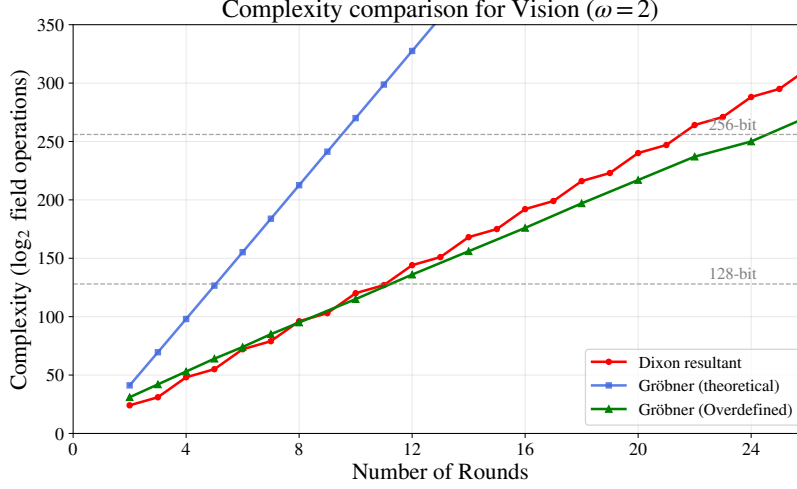
Fig. 4: Complexity comparison for Vision ( \omega = 2 for consistency with [61]).
