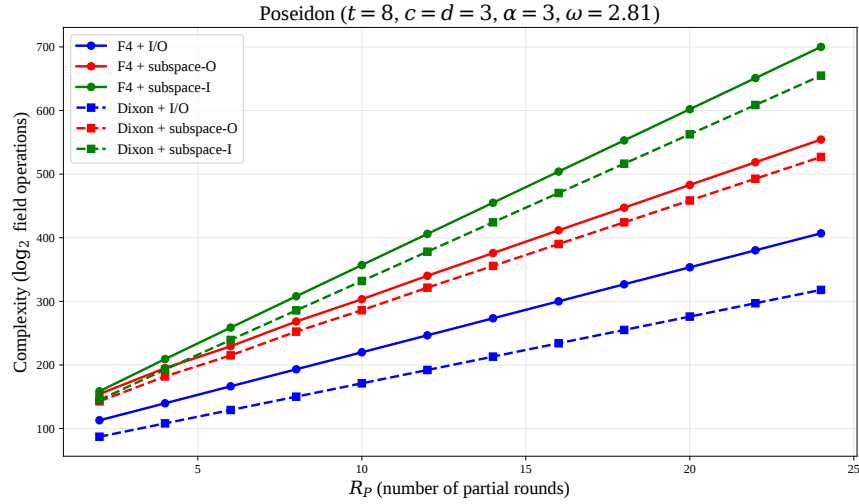
Fig. 3: Complexity comparison for POSEIDON and POSEIDON2, with the model parameters t = 8 , c = d = 3 , \alpha = 3 of [42]. Here \omega = 2.81 for all curves.
