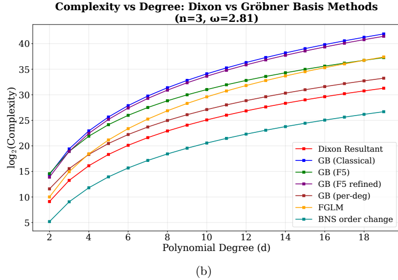
Fig. 6: Complexity comparison between the Dixon resultant and Gröbner basis
