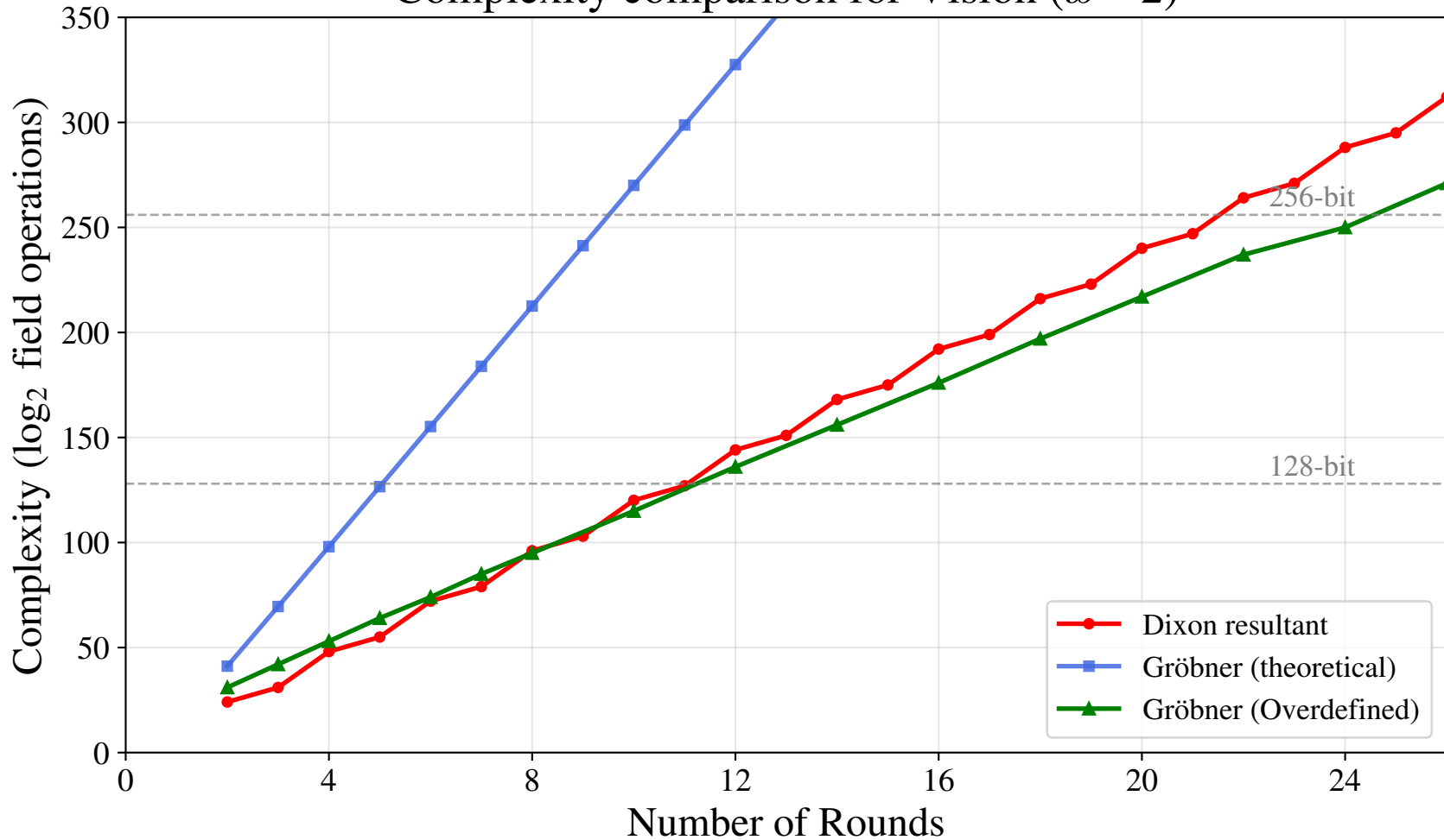
Complexity comparison for Vision ( \omega = 2 )
