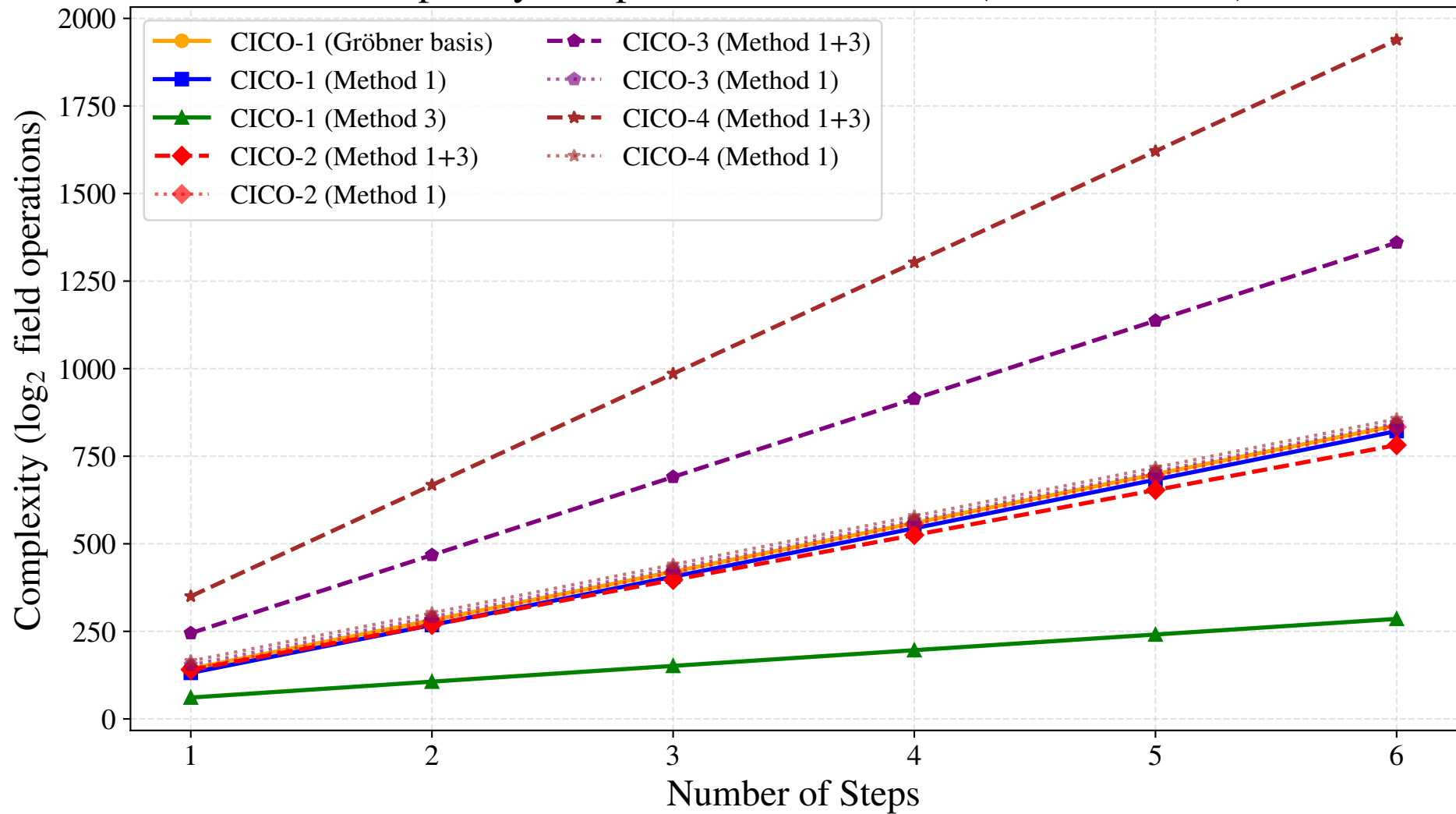
Complexity comparison for XHash12 ( \alpha=7 , \omega=2.81 )
