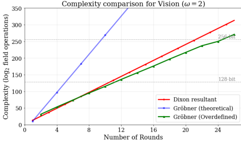
Fig. 4: Complexity comparison for Vision ( \omega = 2 for consistency with [57]).
