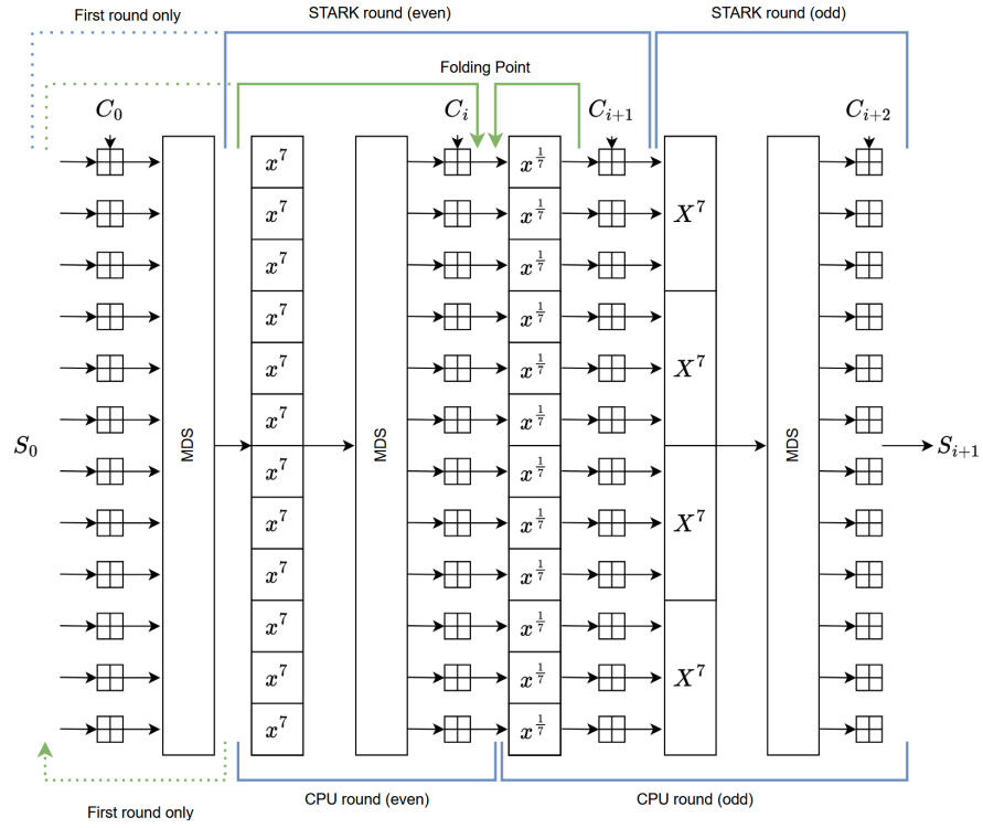
Fig. 11: Round function of XHash12 [5]
