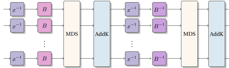
Fig. 10: Round function of Vision . (Figure from [22])
