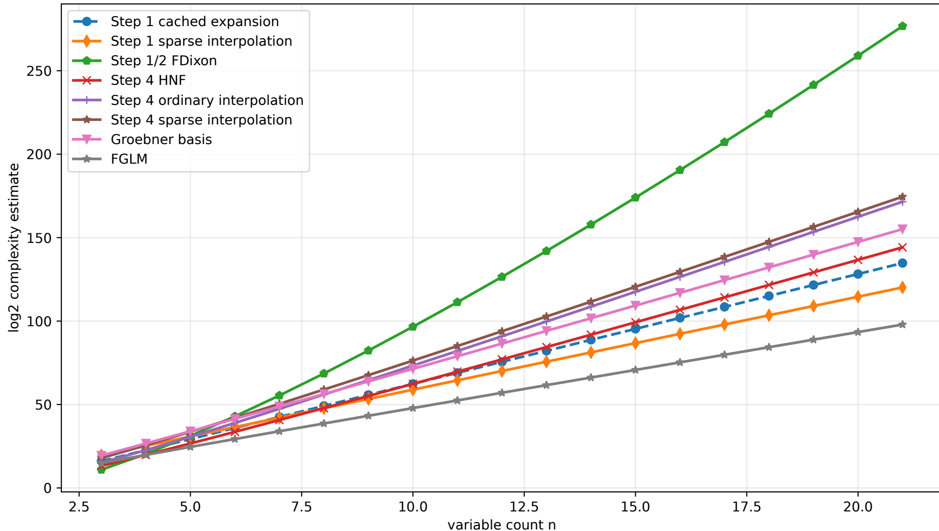
Equal-degree Dixon model: complexity vs variable count ( d=3 , \omega=2.81 )
