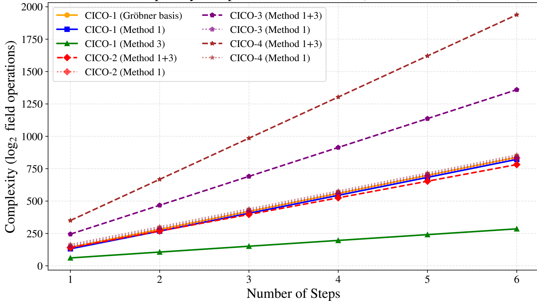
Complexity comparison for XHash12 ( \alpha=7 , \omega=2.81 )
