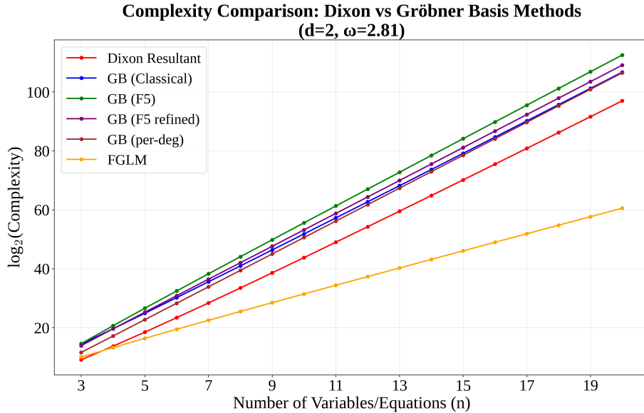
Fig. 1: Complexity comparison varying n with d = 2, \omega = 2.81 . The y-axis shows \log_2(\text{complexity}) . All Gröbner-basis variants tabulated in Table 2, including the GB (per-degree) bound, are included for direct empirical comparison with Dixon.
