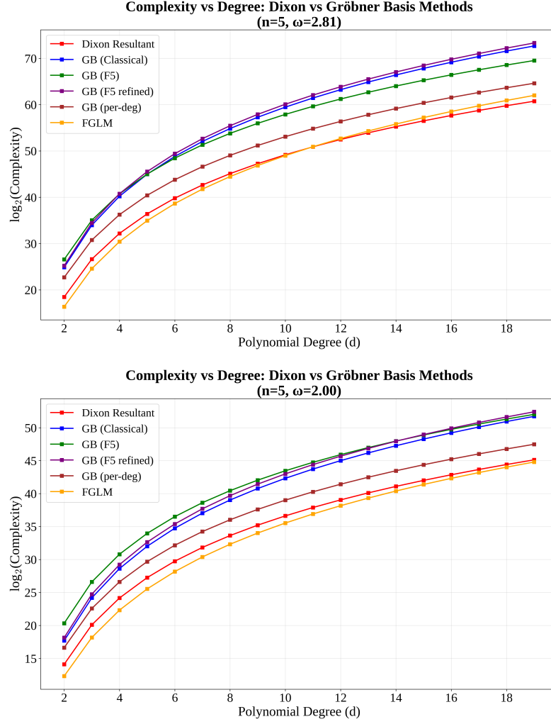
Figure 6 (continued). The bottom panel uses \omega = 2 , at which the first and the final determinant have the same asymptotic order in M ; the plotted Dixon curve is the Step 4 term.
