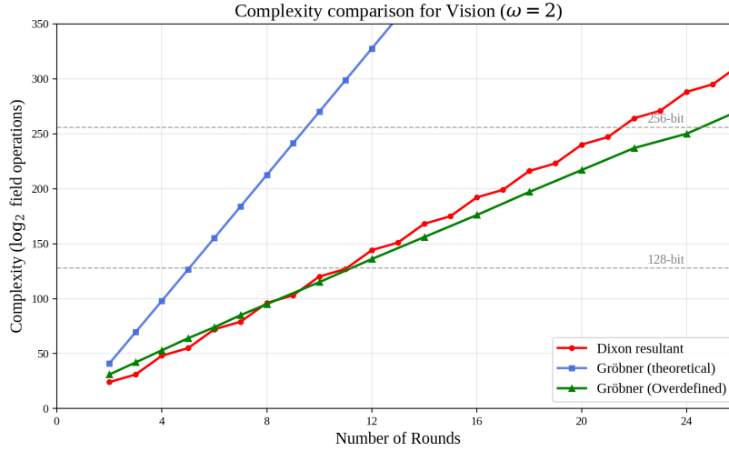
Fig. 4: Complexity comparison for Vision ( \omega = 2 for consistency with [59]).
