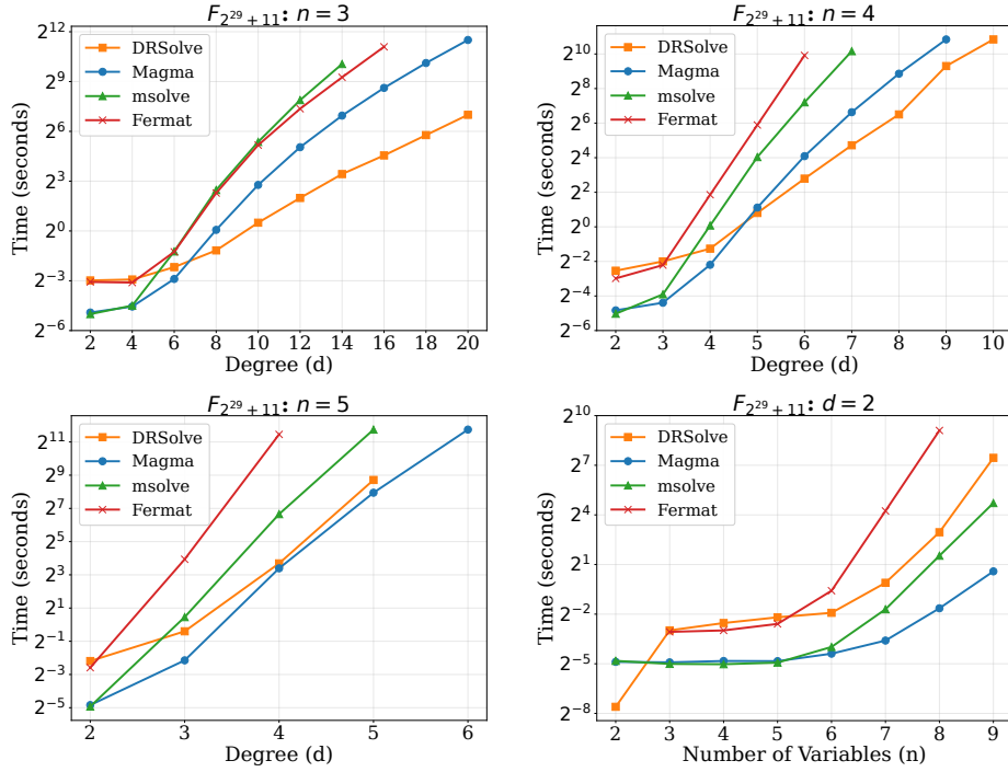
Fig. 1. Performance comparison (time in seconds) of DRSolve 0.3.0, Magma 2.29-7, msolve 0.9.5, and Fermat 7.9b on randomly generated dense polynomial systems over \mathbb{F}_p with p = 2^{29} + 11 . The four panels show degree sweeps for n = 3, 4, 5 and a variable-count sweep for d = 2 ; here n denotes the number of variables (equal to the number of equations). A curve stops where the corresponding solver exceeded one hour.
