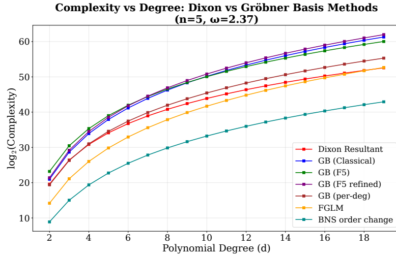
Fig. 6 (continued). The bottom panel uses \omega = 2.37 . Since the asymptotic dominance of the final determinant sets in only for larger (n, d) than those plotted, the Dixon curve of this panel reports the maximum over the two symbolic stages, \max\{T_1^{\text{best}}, T_4^{\text{best}}\} , which over this range is governed by Step 1.
