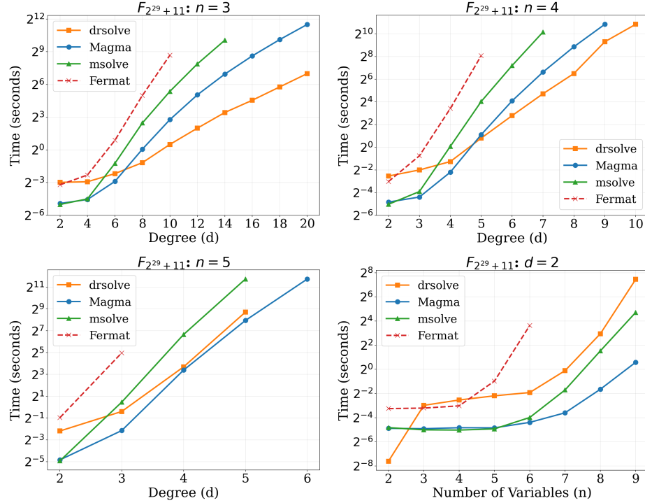
Fig. 2: Performance comparison (time in seconds) of DRsolve, Magma, msolve, and Fermat on randomly generated dense polynomial systems over \mathbb{F}_{2^{29}+11} . The four panels show degree sweeps for n = 3, 4, 5 and a variable-count sweep for d = 2 ; here n denotes the number of variables (equal to the number of equations).
