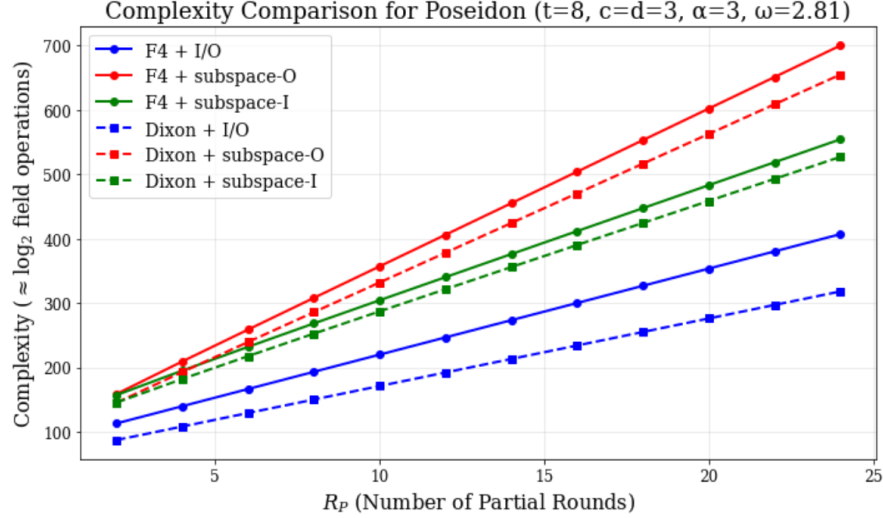
Fig. 3: Complexity comparison for POSEIDON and POSEIDON2 ( t = 8 , c = d = 3 , \alpha = 3 ). Here \omega = 2.81 for all curves.
