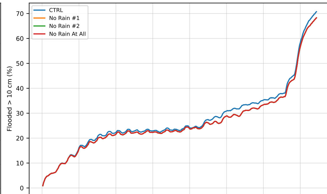
Areal Flooding Fraction - New Experiments (Aug-Sep 1905)
