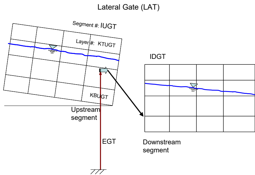
Figure 17. Lateral gate LAT designation.
