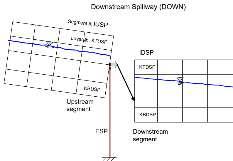
Figure 14. Downstream spillway DOWN designation. Lateral Spillway (LAT)
