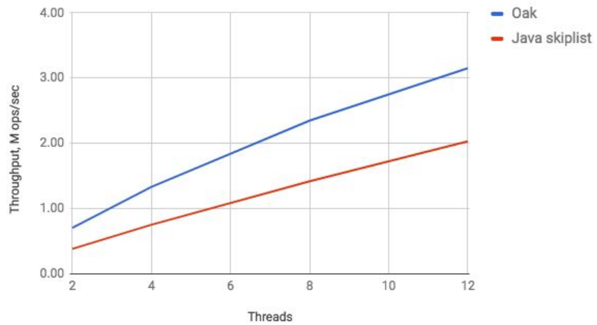
Put + Remove
