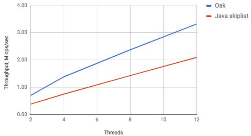
PutIfAbsent + Remove
