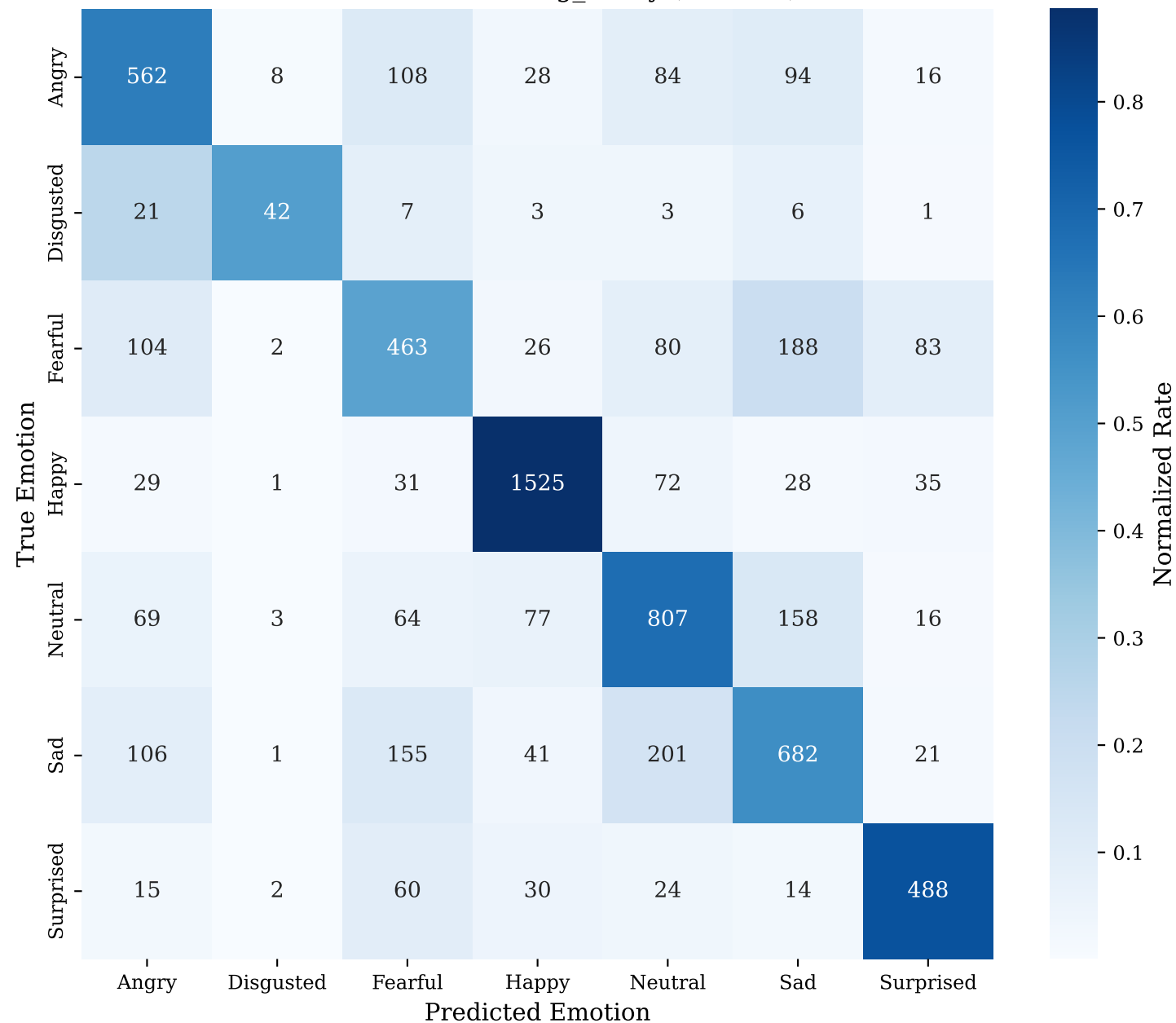
Confusion Matrix: aug_heavy (Test Set)
