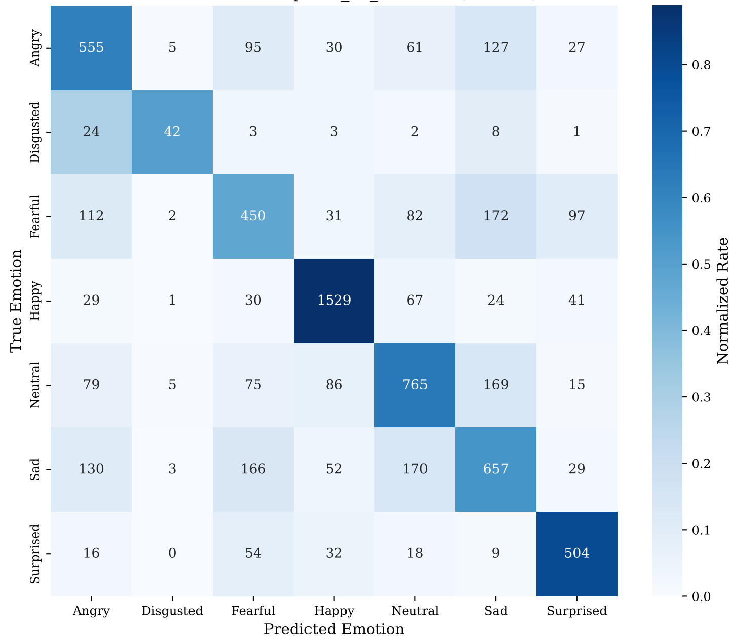
Confusion Matrix: epochs_50_extended (Test Set)
