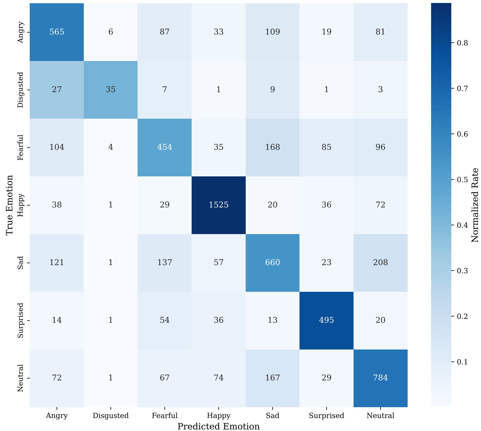
Confusion Matrix: Custom-ResNet18
