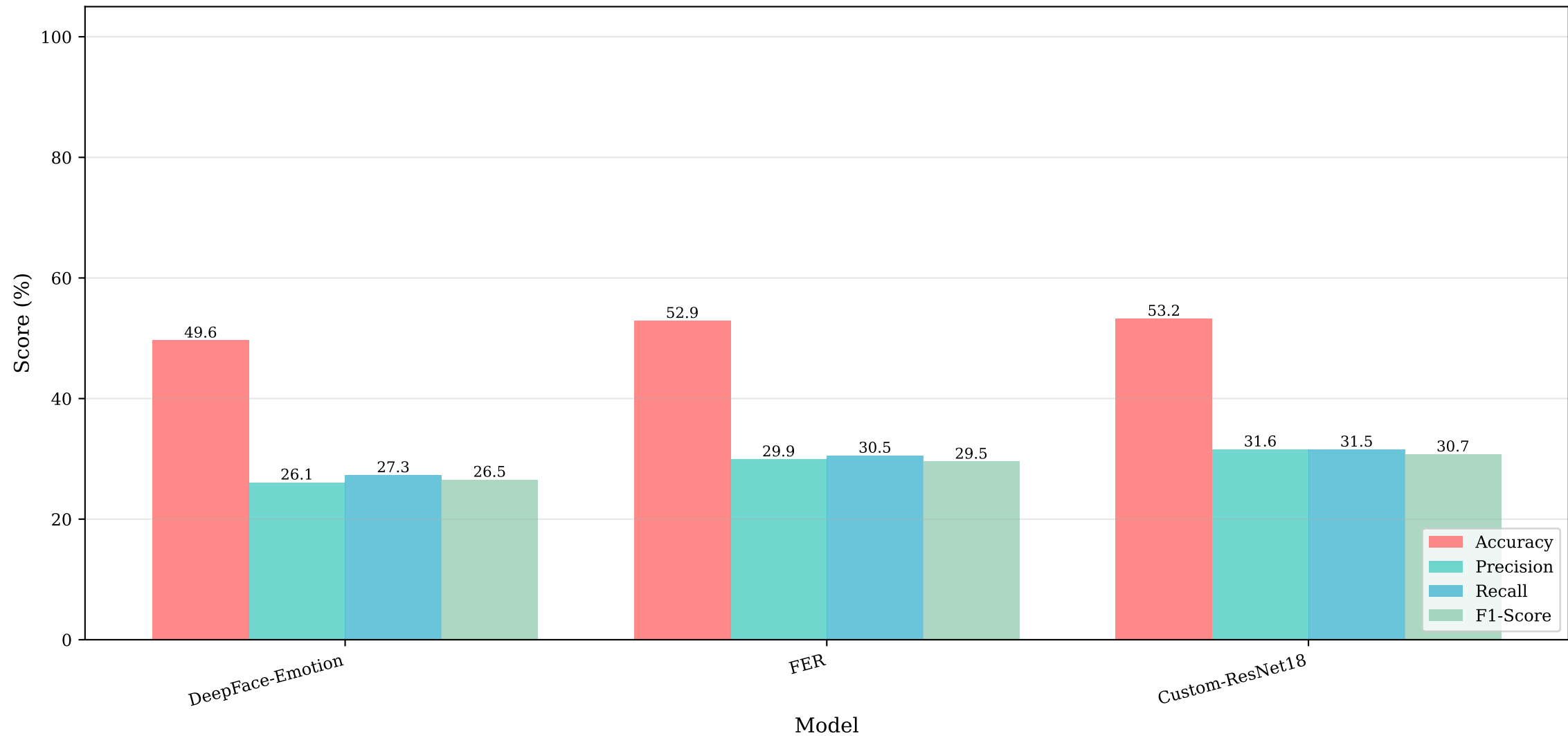
Overall Model Performance on GREYSCALE Dataset 3 Test Set
