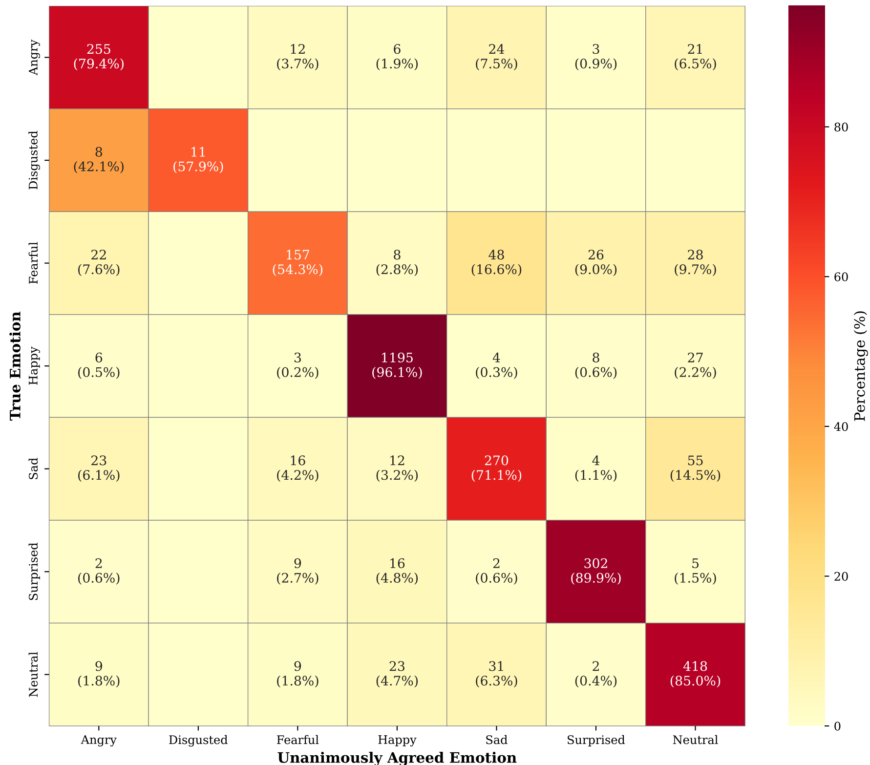
Agreement Confusion Matrix (When All Models Agree, What Do They Predict vs. True Label)
