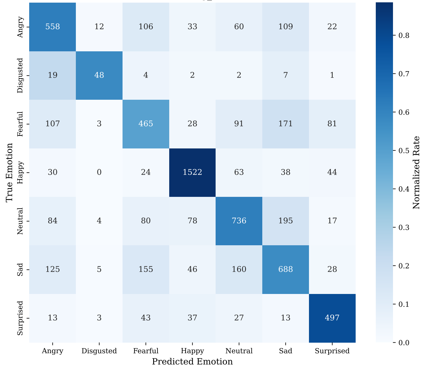
Confusion Matrix: aug_none (Test Set)
