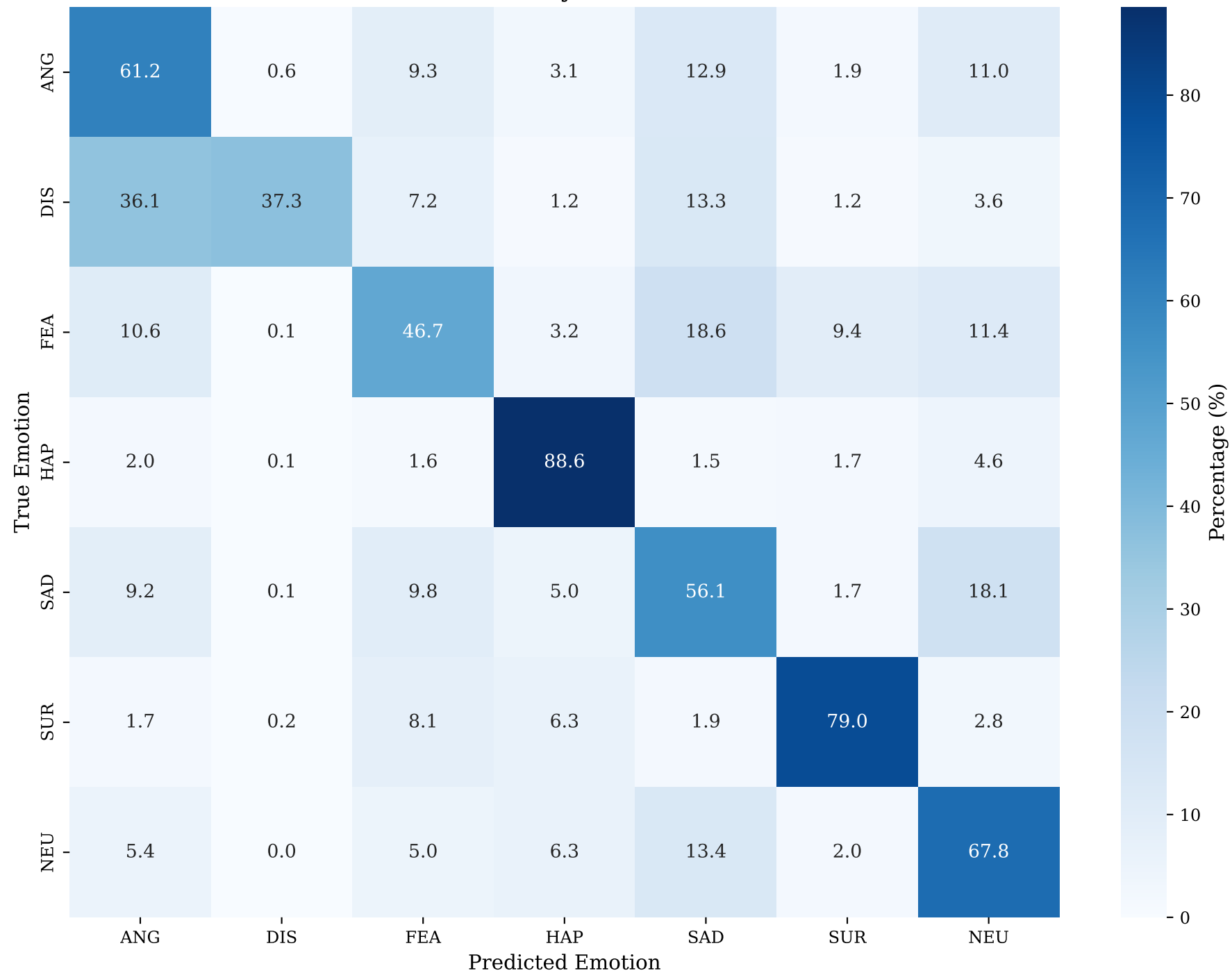
Ensemble Confusion Matrix (Faces_Dataset)
