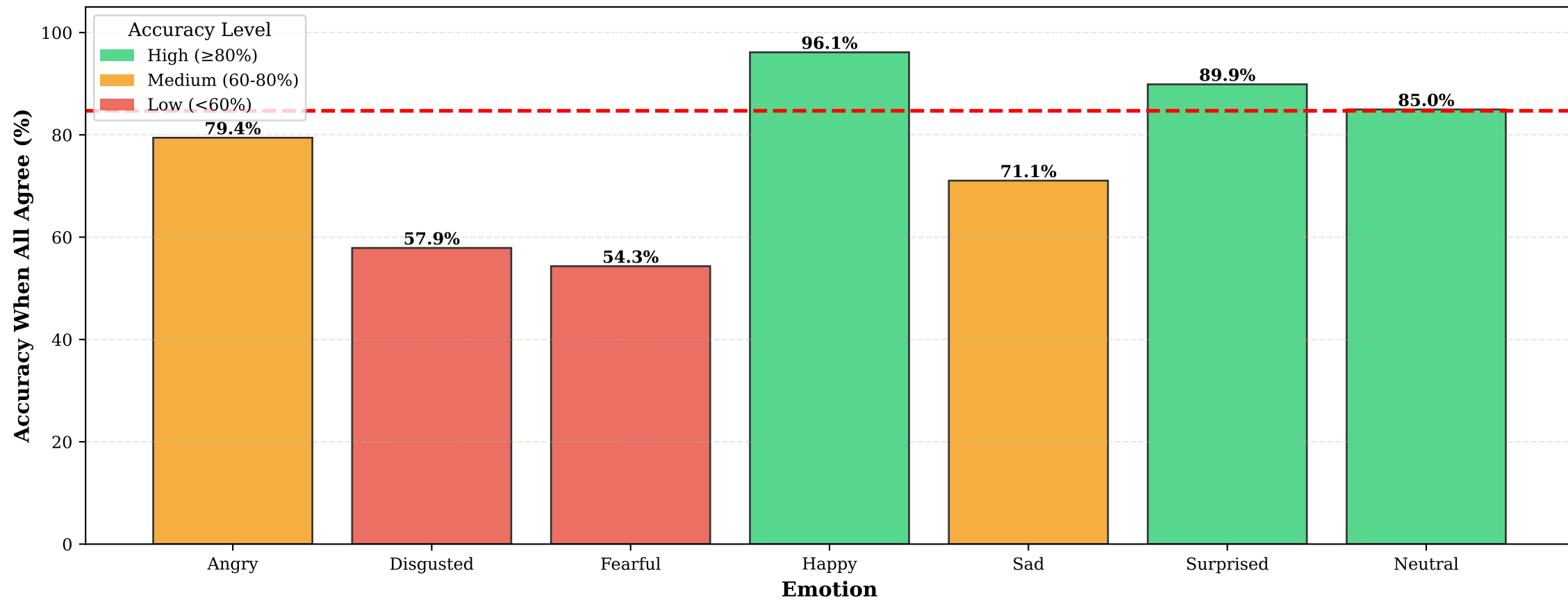
Prediction Correctness When All 3 Models Agree
