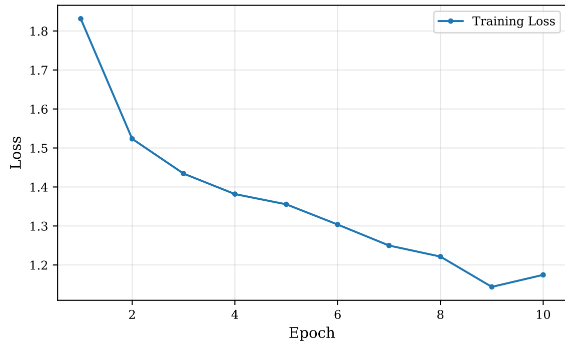
Loss Curves
