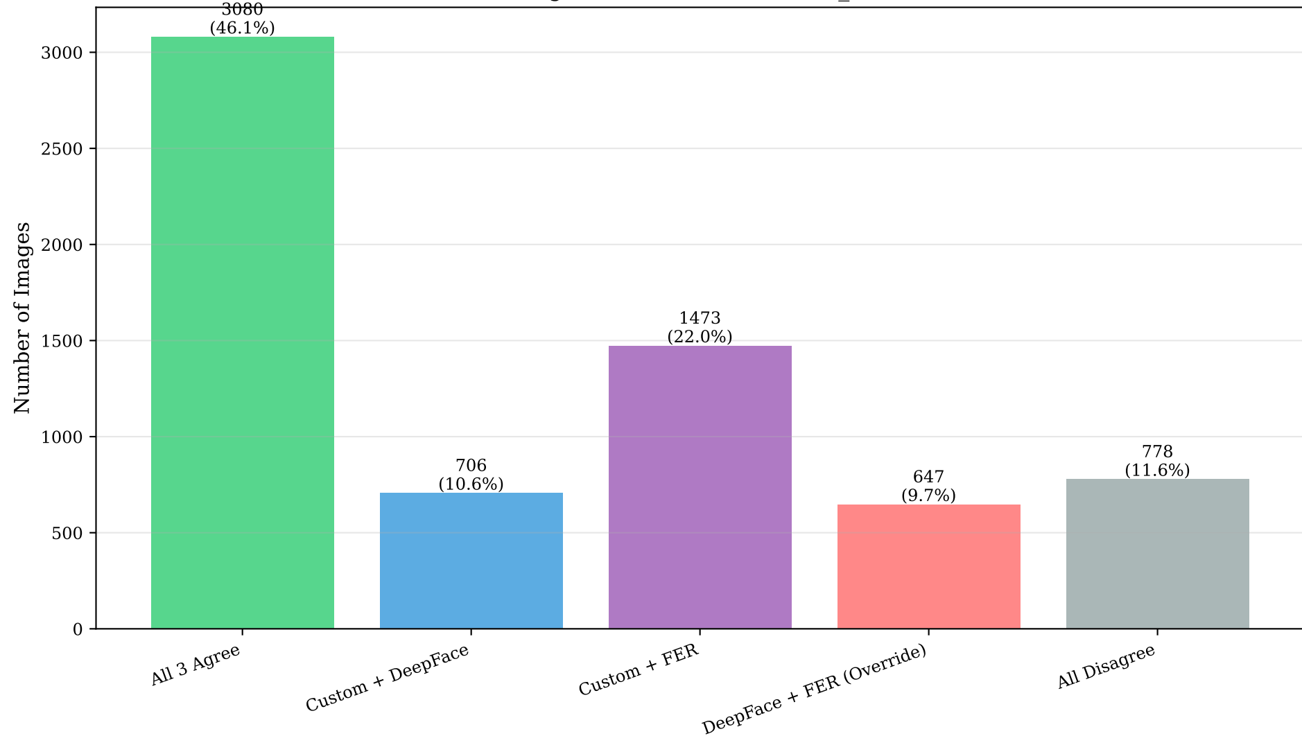
Model Agreement Patterns (Faces_Dataset)
