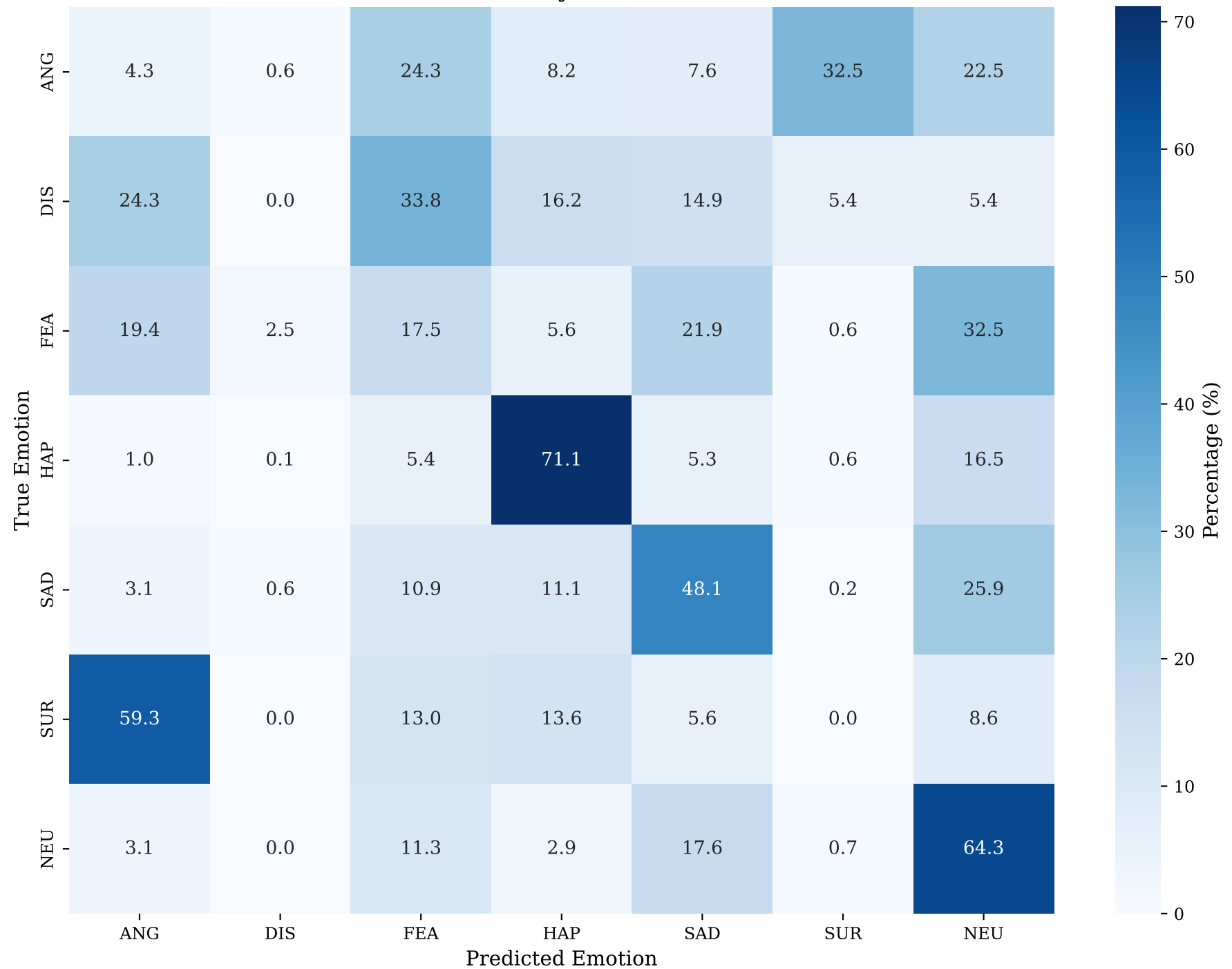
Ensemble Confusion Matrix Accuracy: 50.6%
