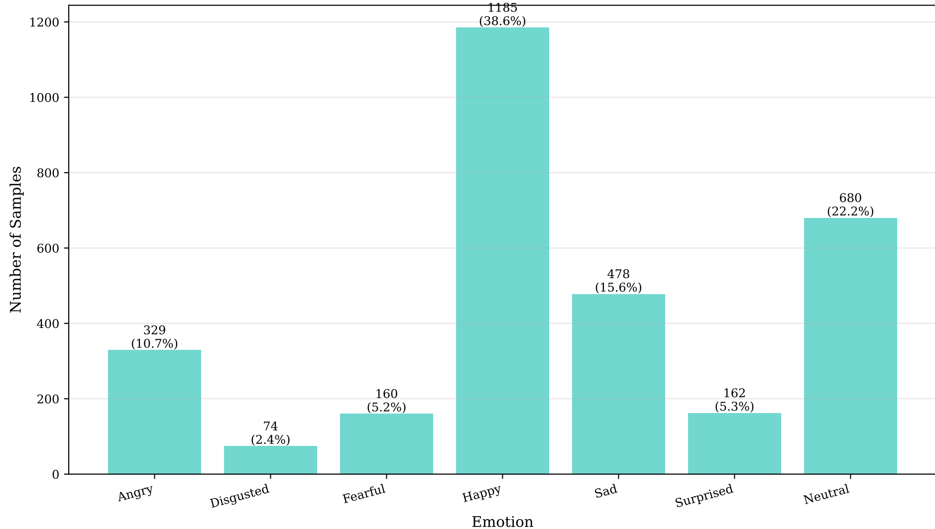
Class Distribution in Dataset 3 Test Set (Total: 3068)
