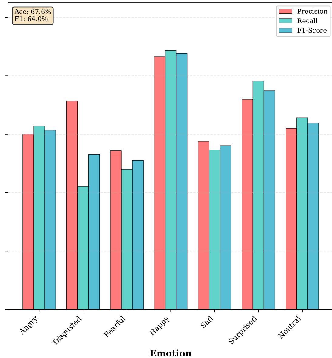
Custom-ResNet18
