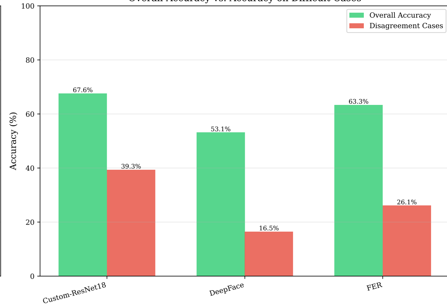
Overall Accuracy vs. Accuracy on Difficult Cases
