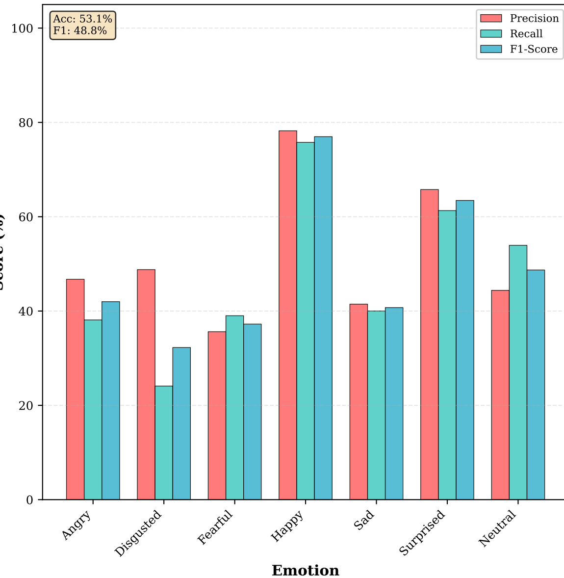
DeepFace-Emotion
