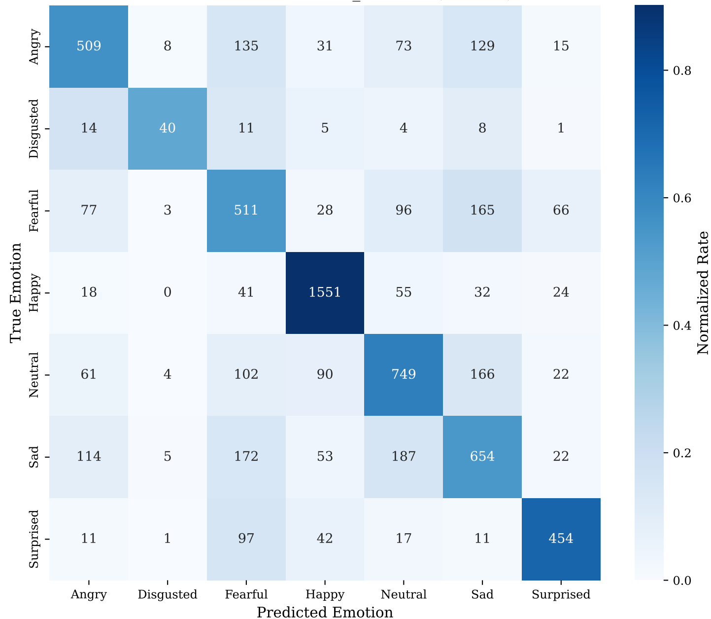
Confusion Matrix: baseline_resnet18 (Test Set)
