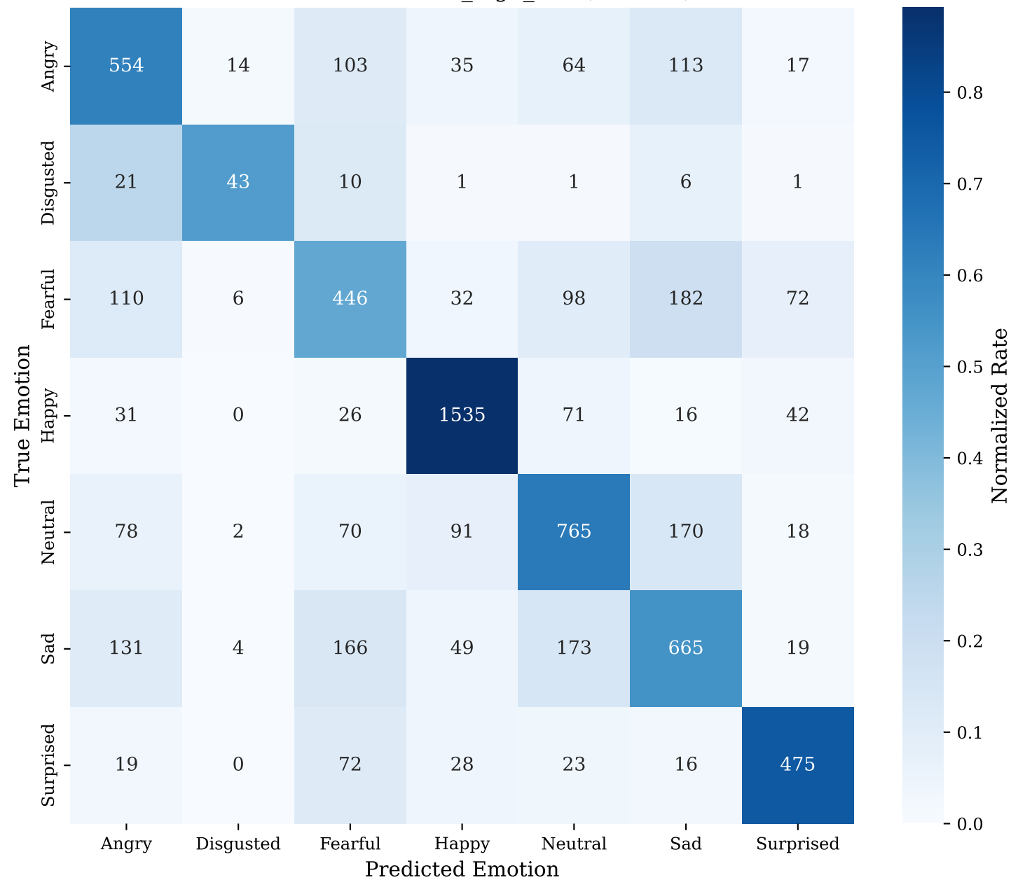
Confusion Matrix: lr_high_1e3 (Test Set)
