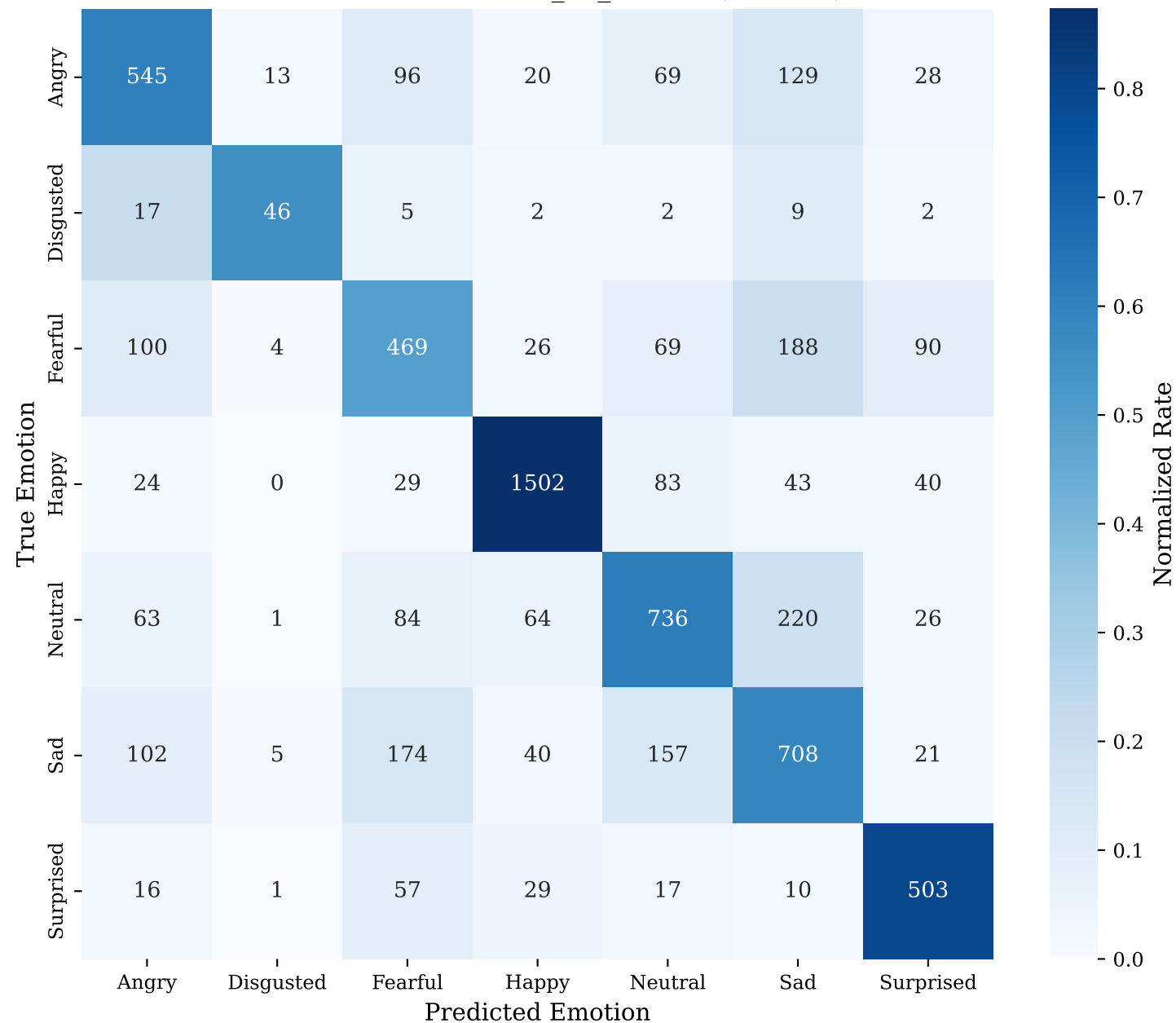
Confusion Matrix: batch_64_smaller (Test Set)
