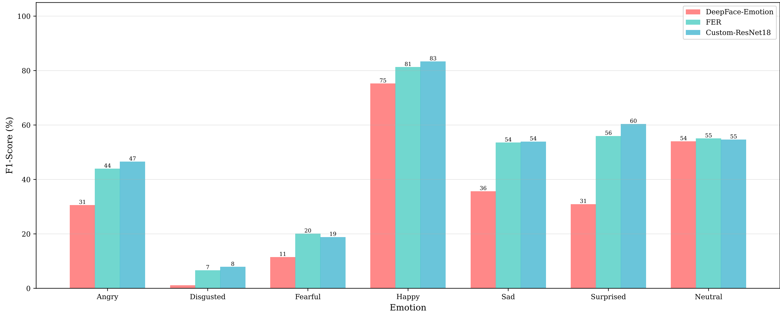
Per-Emotion F1-Score Comparison - GREYSCALE Dataset 3 Test Set
