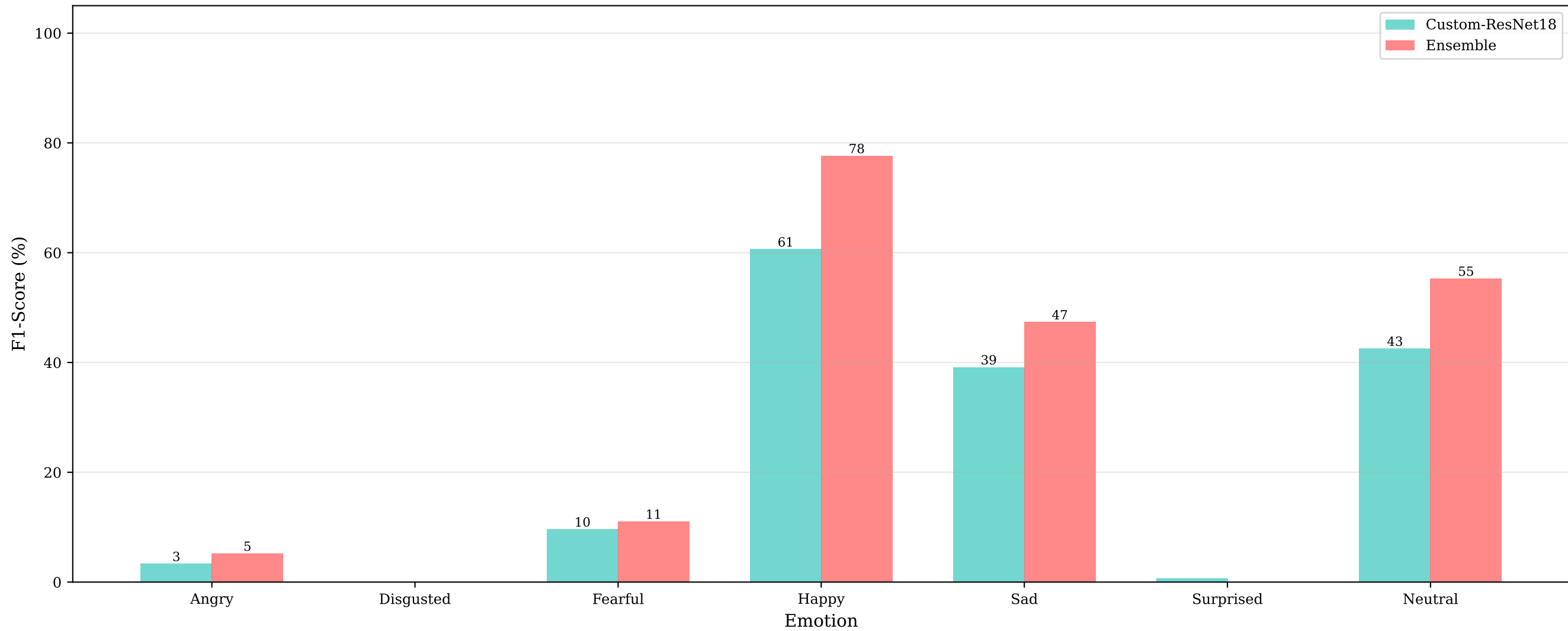
Per-Emotion F1-Score: Custom-ResNet18 vs. Ensemble
