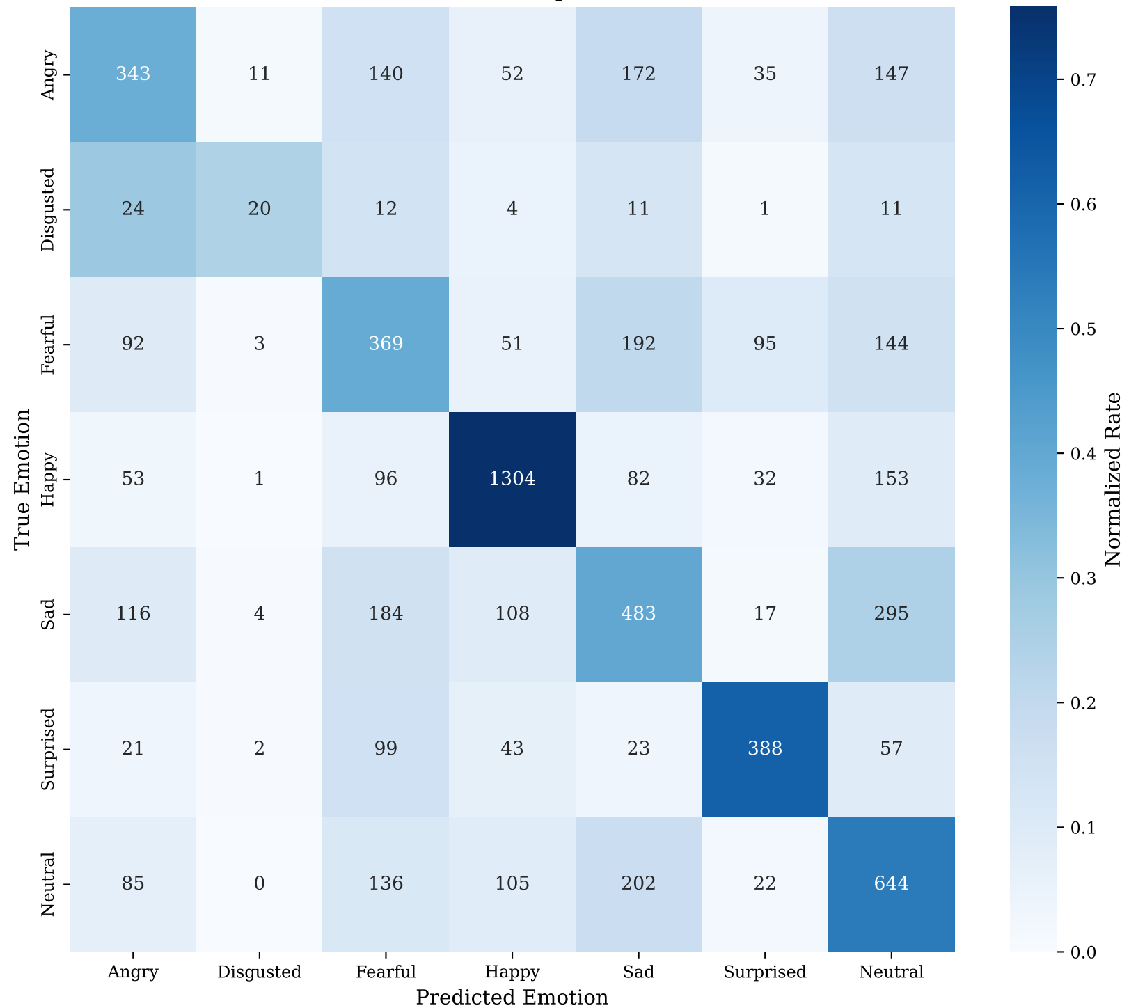
Confusion Matrix: DeepFace-Emotion
