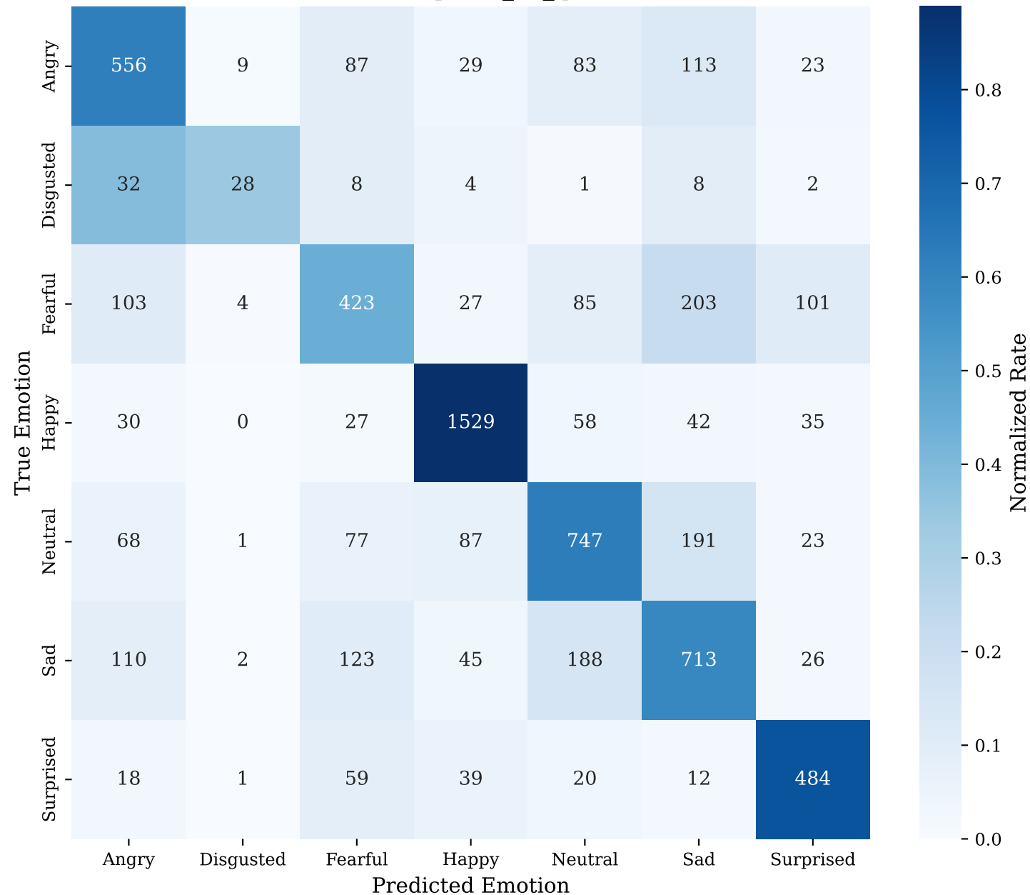
Confusion Matrix: epochs_10_quick (Test Set)
