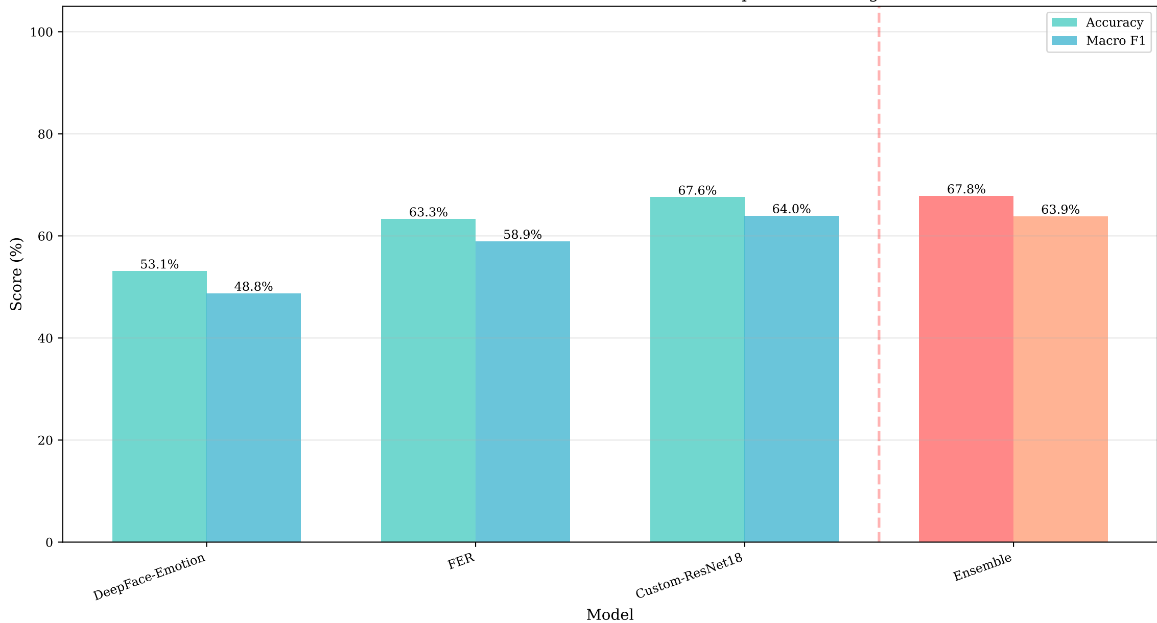
Performance Comparison: Individual Models vs. Ensemble (Faces Dataset) Ensemble: Custom-ResNet18 + Override when DeepFace & FER Agree
