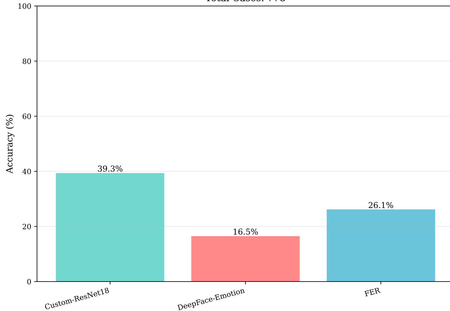
Performance on Difficult Cases (All Models Disagree)
