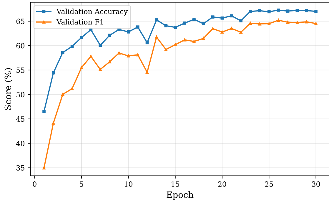
Accuracy and F1 Curves
