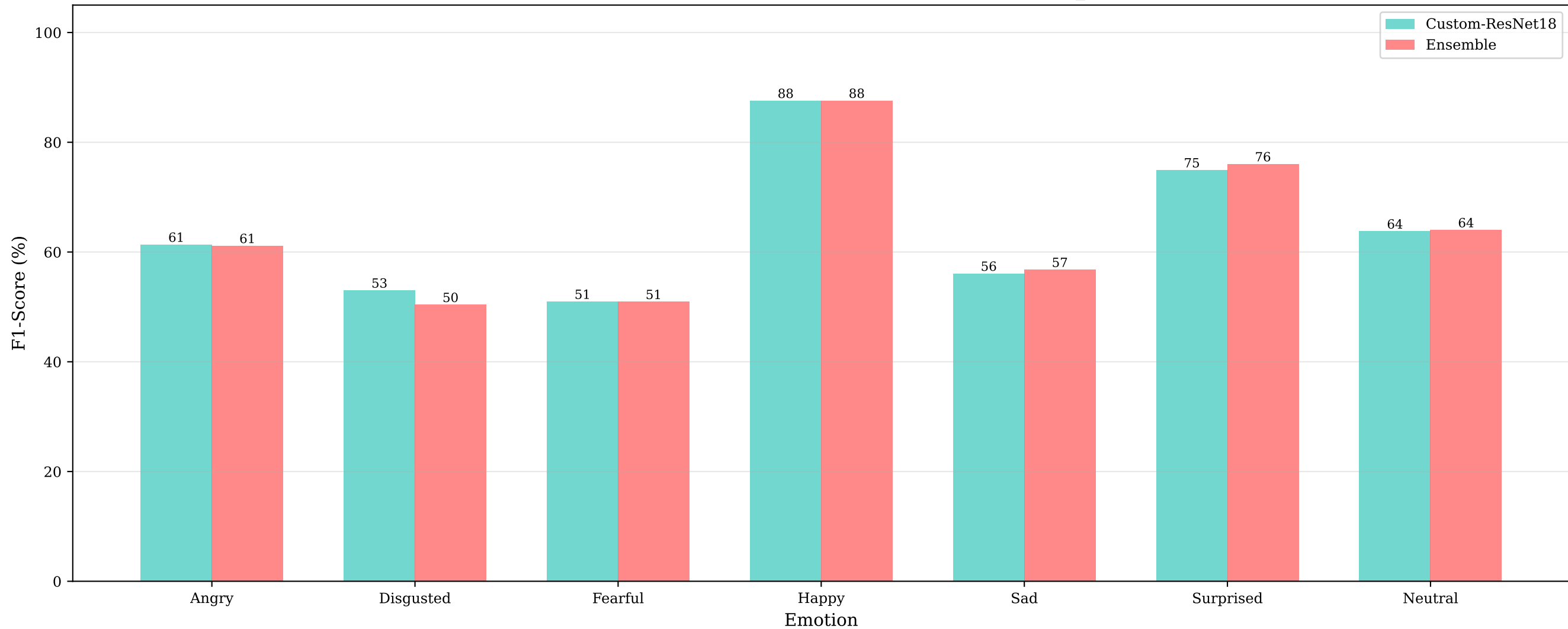
Per-Emotion F1-Score: Custom-ResNet18 vs. Ensemble (Faces_Dataset)
