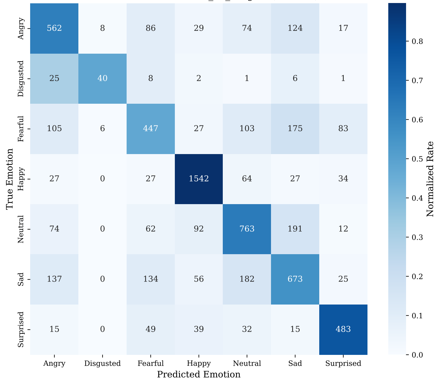
Confusion Matrix: balance_no_weights (Test Set)
