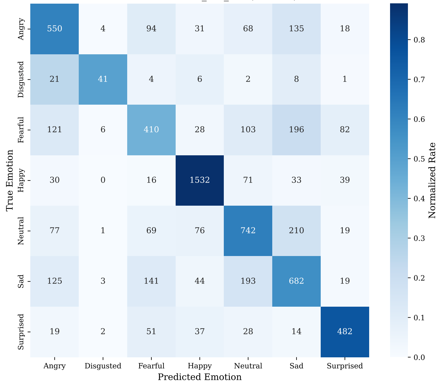
Confusion Matrix: lr_low_1e4 (Test Set)
