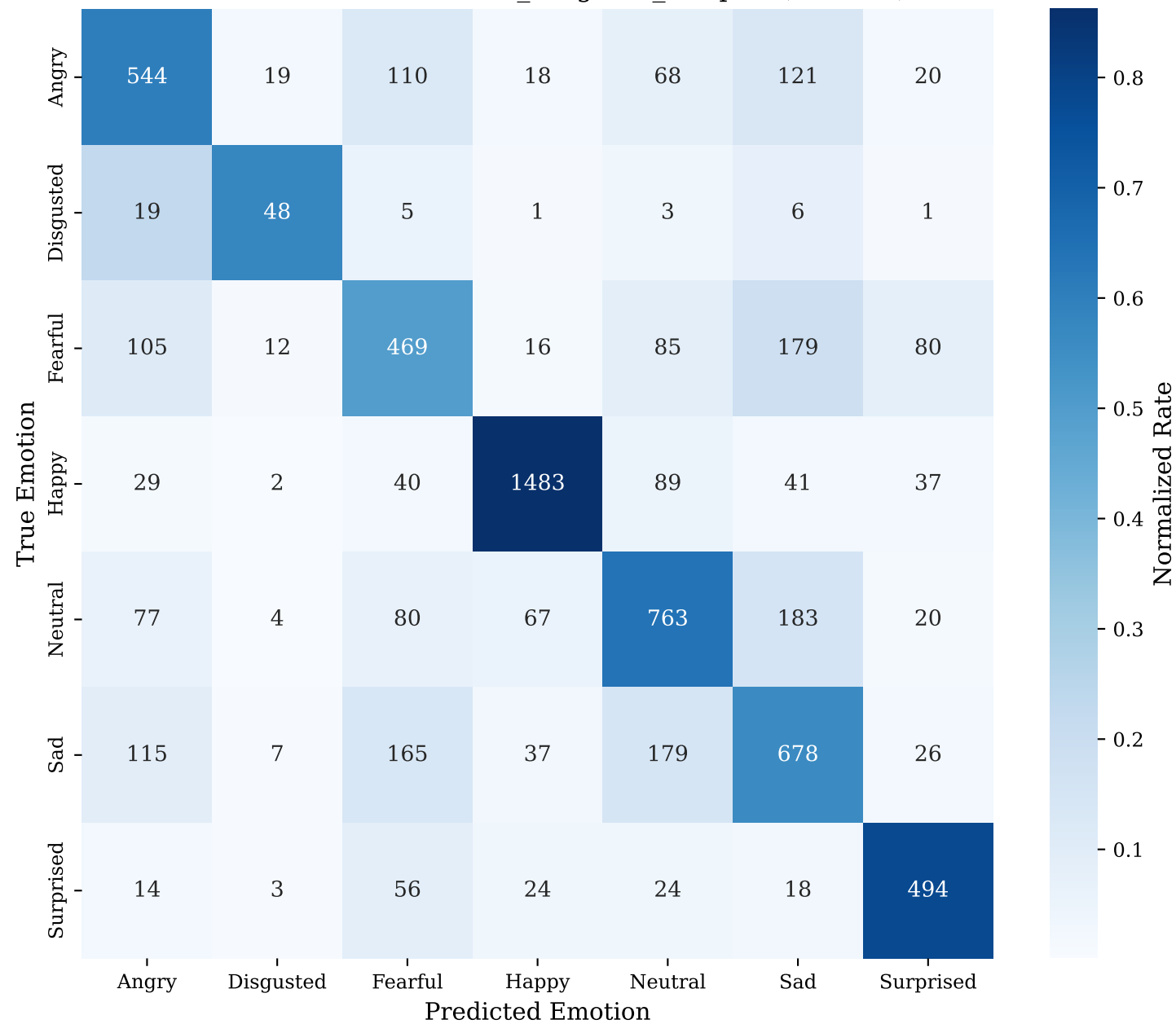
Confusion Matrix: balance_weighted_sampler (Test Set)
