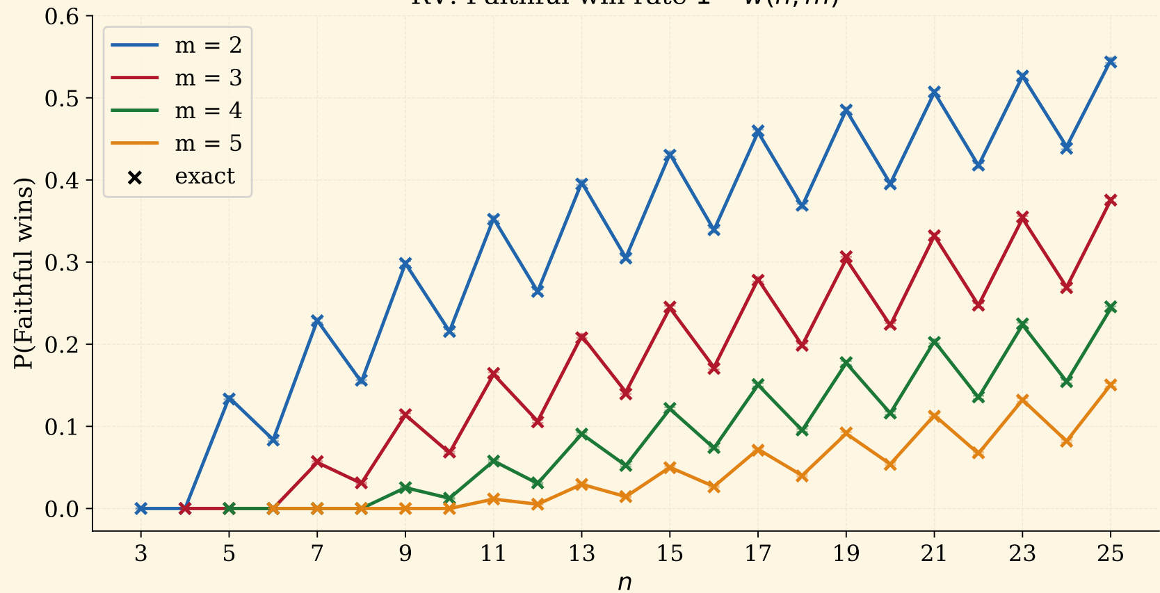
RV: Faithful win rate 1 - w(n, m)
