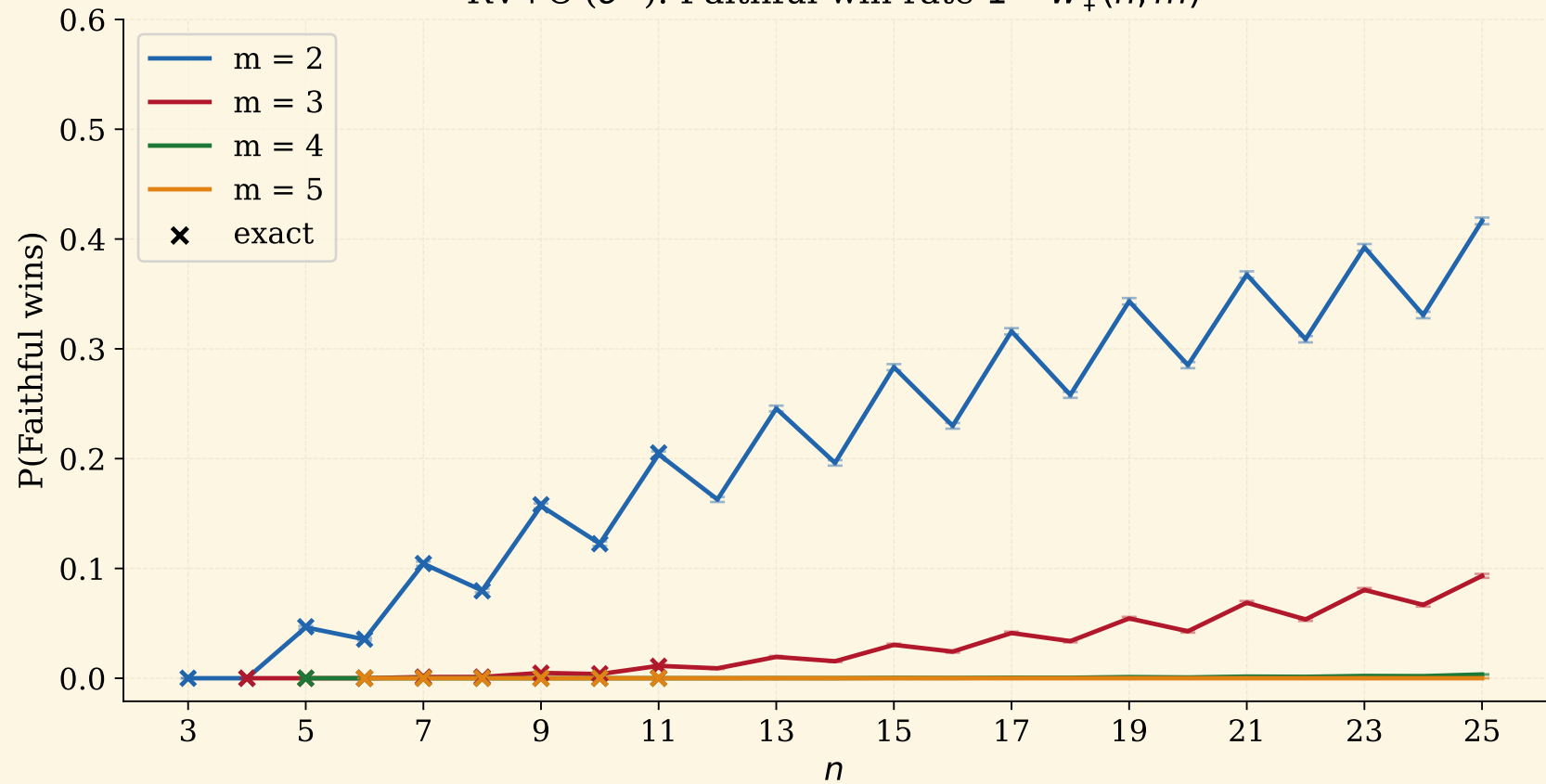
RV+C ( \sigma^\pm ): Faithful win rate 1 - w_+(n, m)
