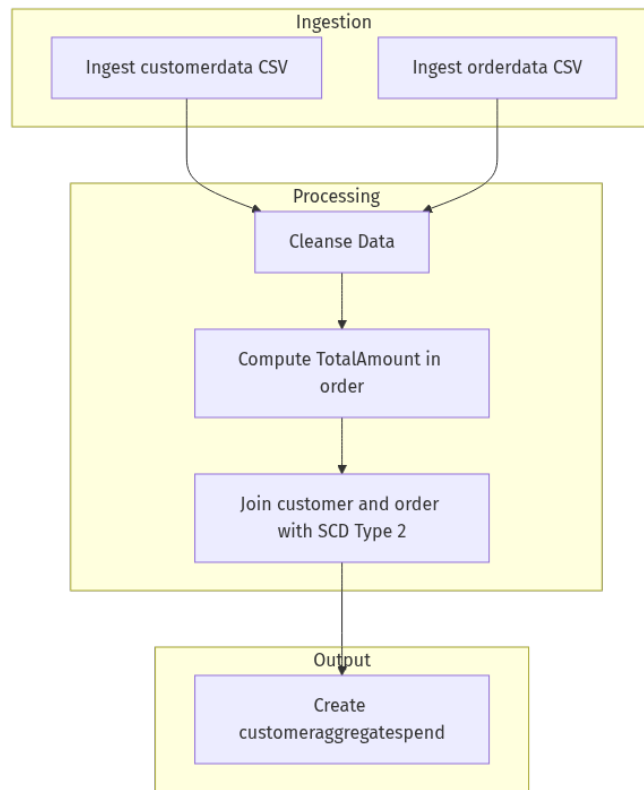
Figure 1: End-to-End Data Pipeline Flow
