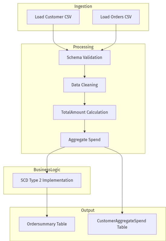
Figure 1: End-to-End Data Pipeline Flow
