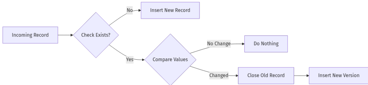
Figure 2: SCD Type 2 Processing Logic
