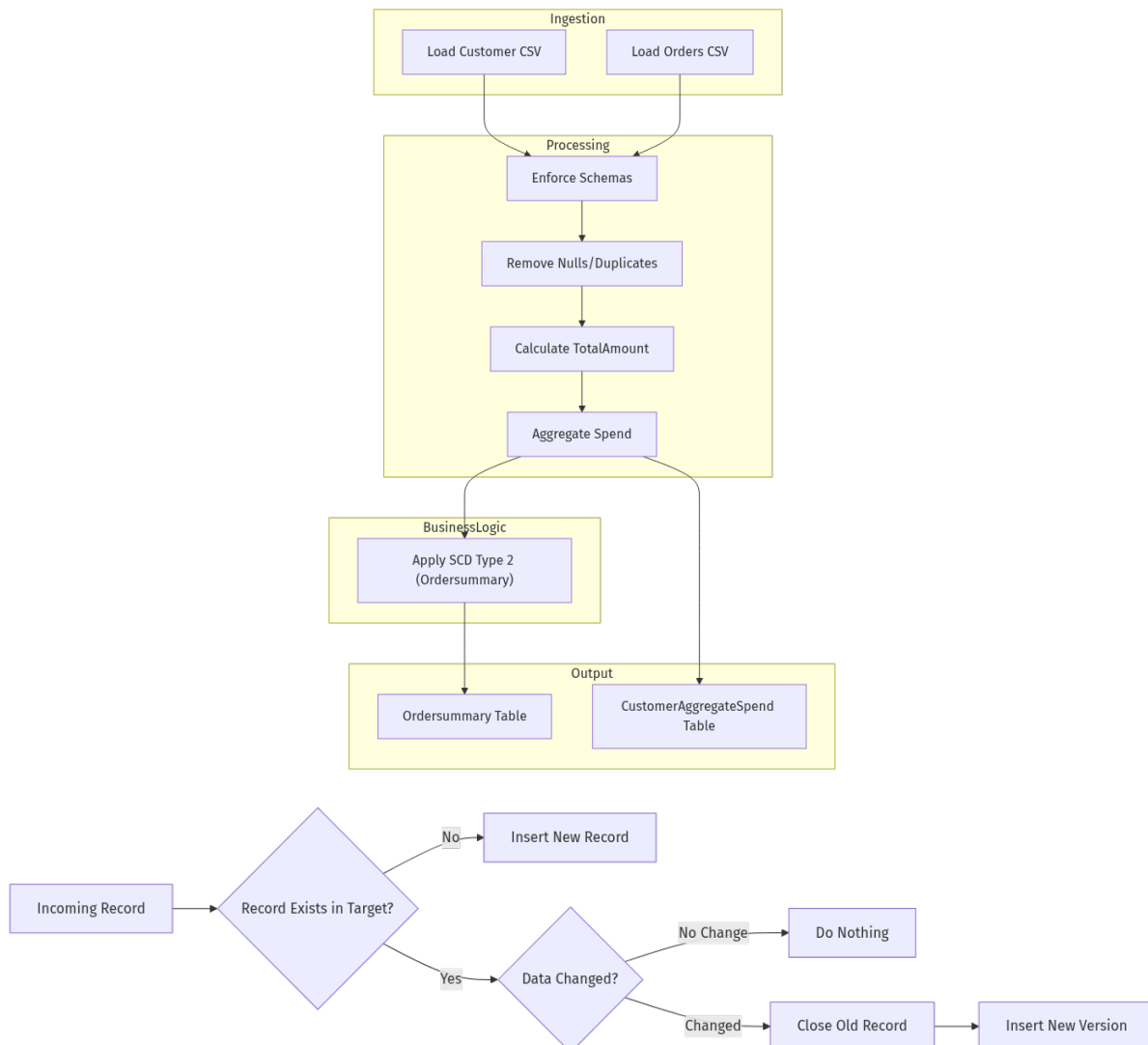
Figure 2: SCD Type 2 Processing Logic
