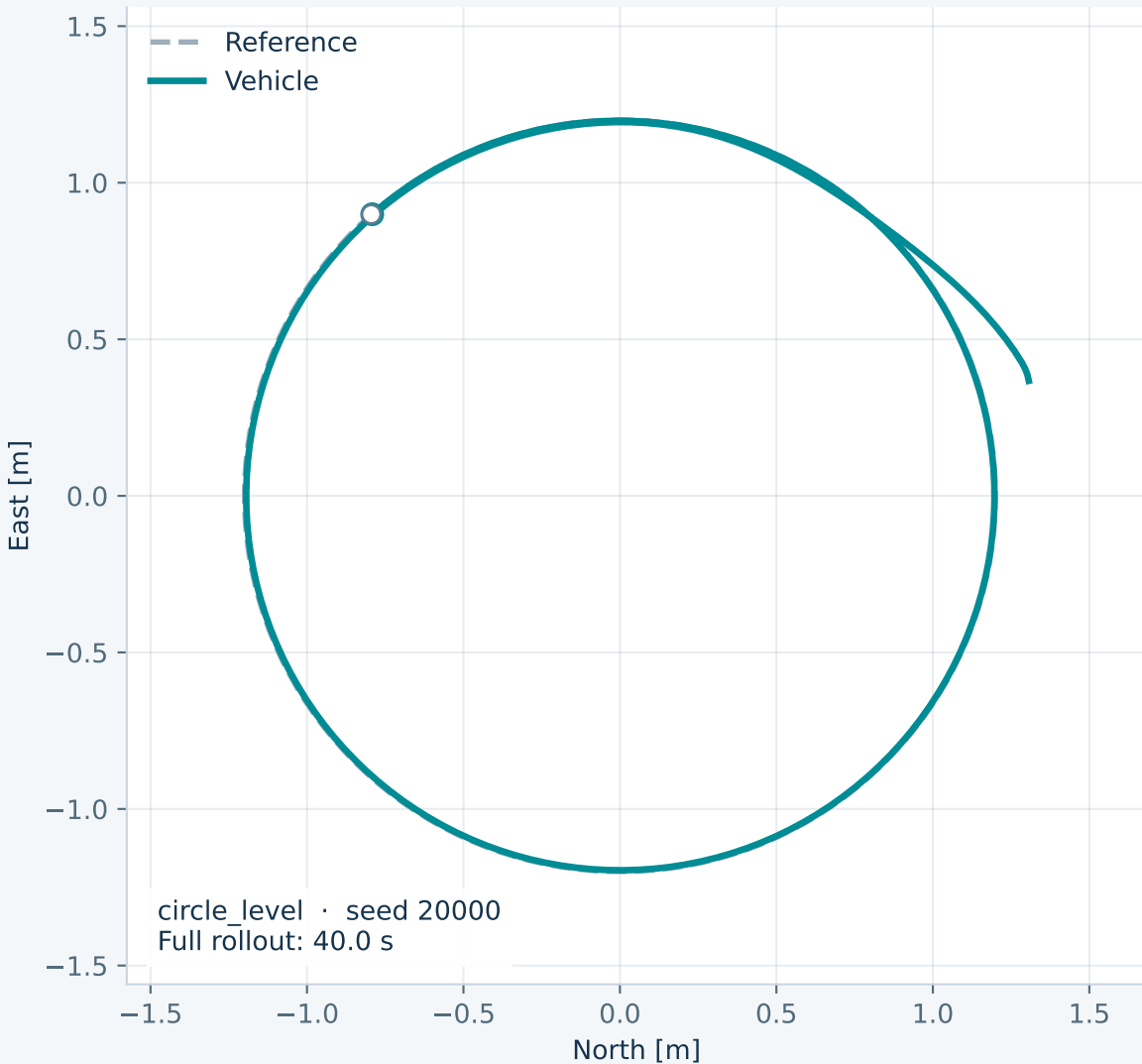
Trajectory tracking · top view
