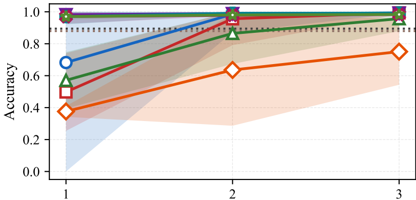
Communication Round
