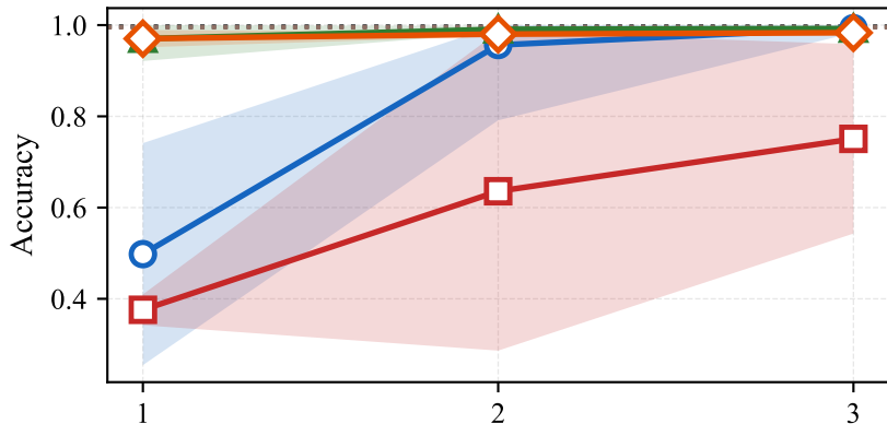
Accuracy — non_iid_label
