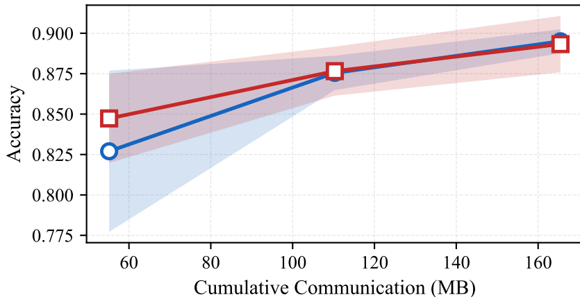
Accuracy vs communication — non_iid_label_sub0.01
