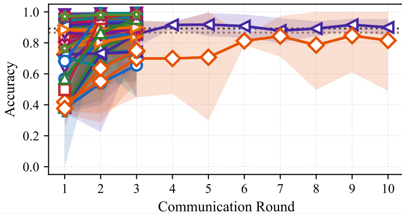
Accuracy — all
