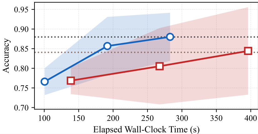
Accuracy vs time — iid_sub0.05
