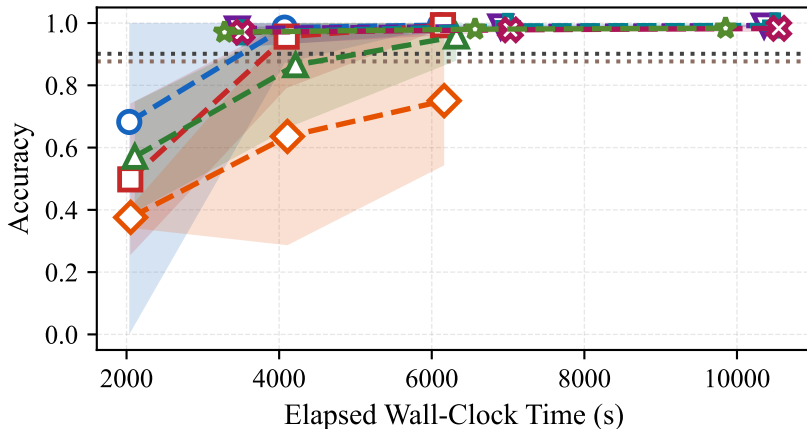
Accuracy vs time — all
