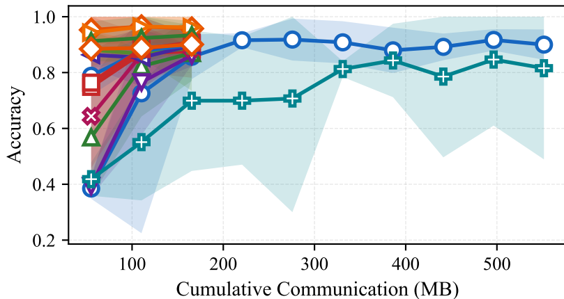
Accuracy vs communication — non_iid_label
