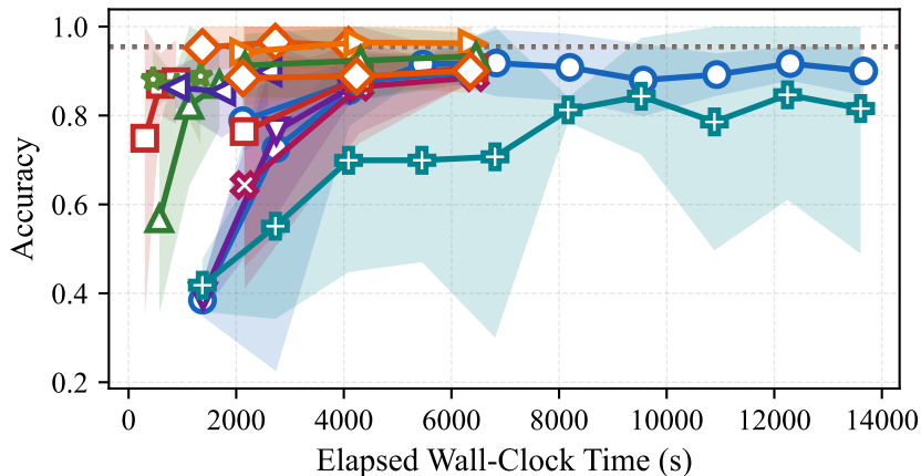
Accuracy vs time — non_iid_label
