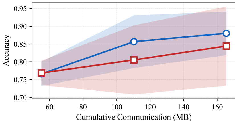
Accuracy vs communication — iid_sub0.05
