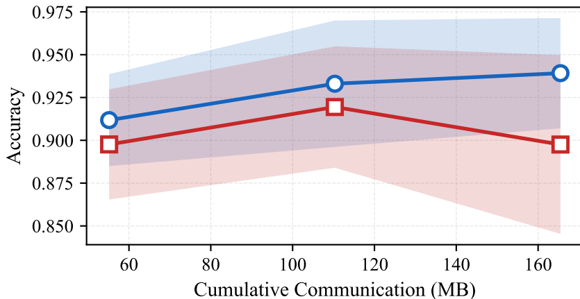
Accuracy vs communication — non_iid_label_sub0.05
