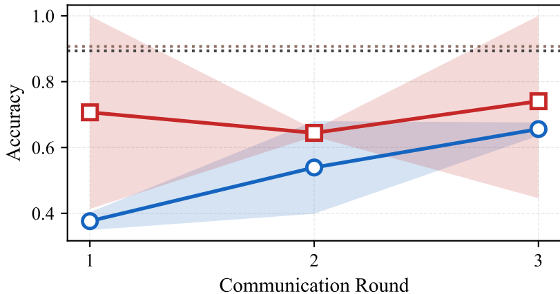
Accuracy — dirichlet_0.1
