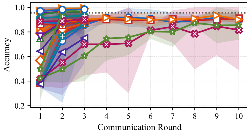
Accuracy — non_iid_label
