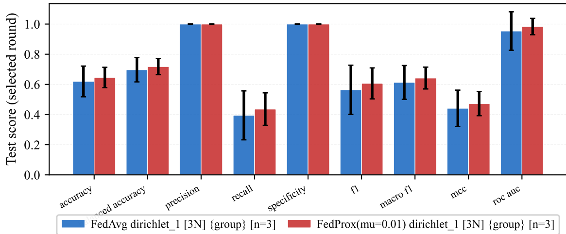
Selected-round test metrics — dirichlet_1
