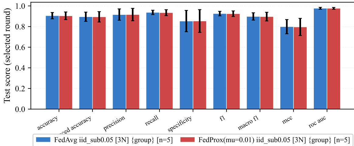
Selected-round test metrics — iid_sub0.05
