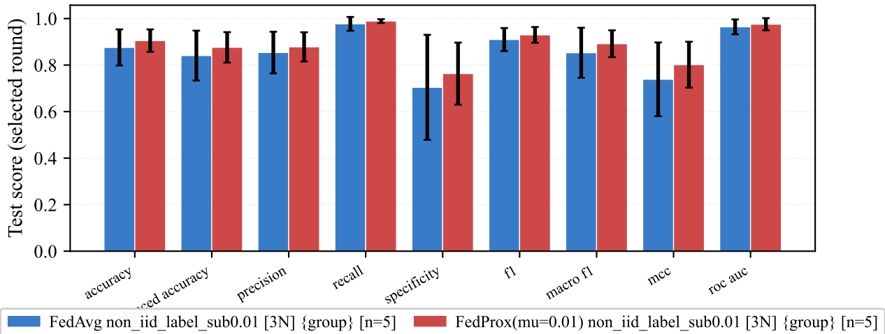
Selected-round test metrics — non_iid_label_sub0.01
