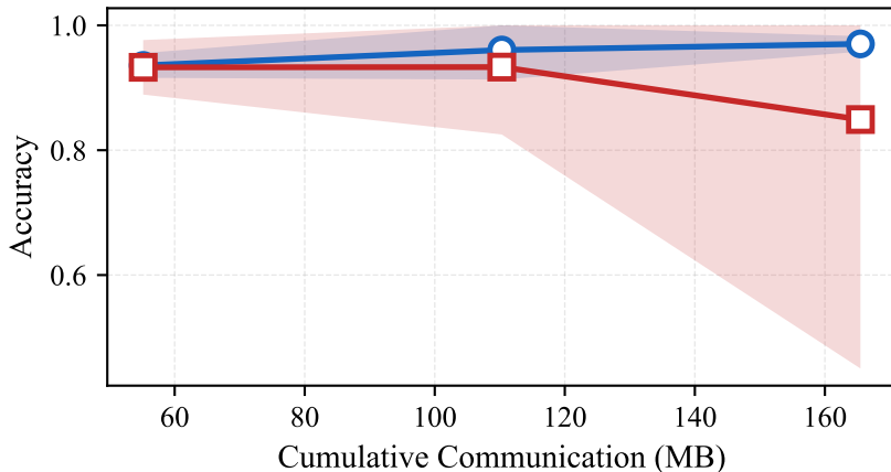
Accuracy vs communication — dirichlet_0.5
