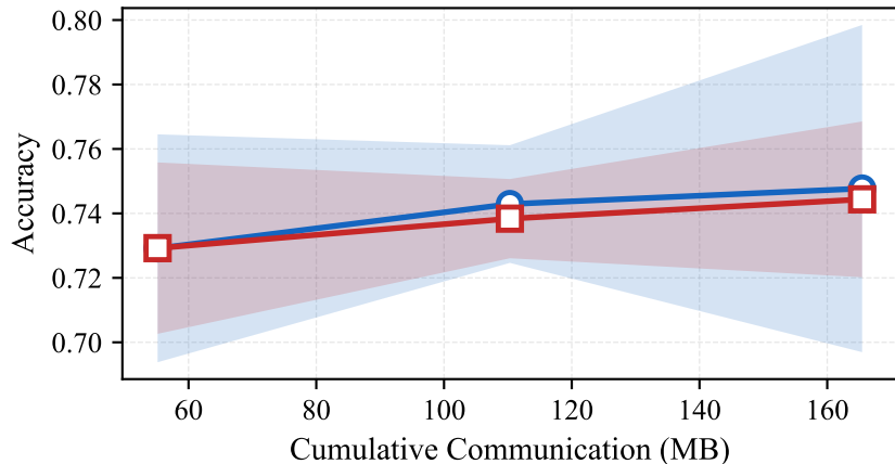
Accuracy vs communication — iid_sub0.01
