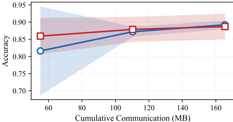
Accuracy vs communication — non_iid_label_sub0.01
