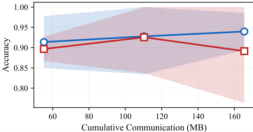
Accuracy vs communication — non_iid_label_sub0.05
