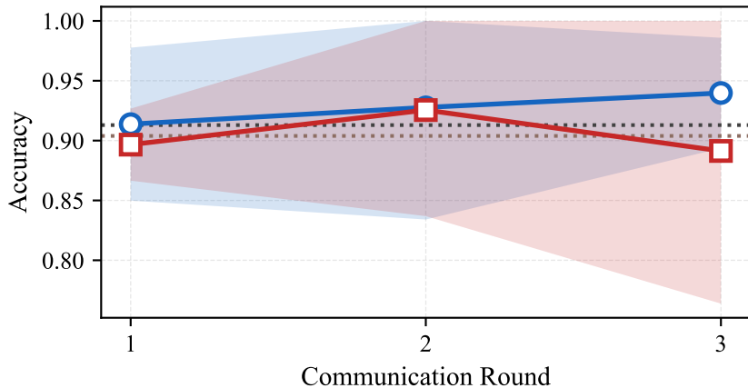
Accuracy — non_iid_label_sub0.05
