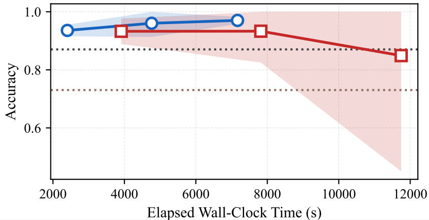
Accuracy vs time — dirichlet_0.5
