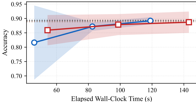
Accuracy vs time — non_iid_label_sub0.01
